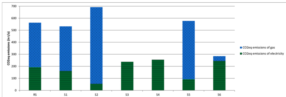
Figure 9. CO 2 eq balance of the total result, by scenario, Variant 3 (increased CO 2 eq emissions of electricity).
