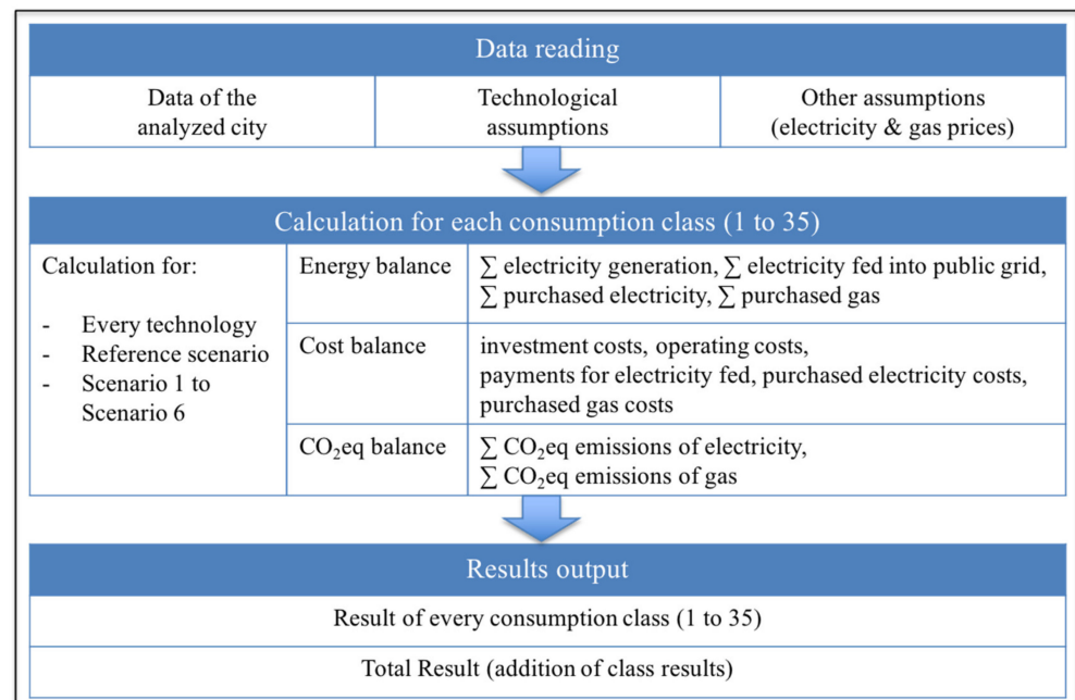
Figure 2. Procedure for the exploitation of the data set.
