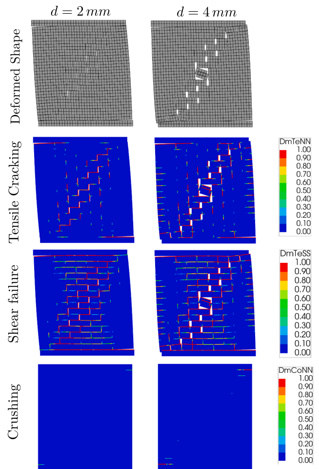
Fig. 8. The deformed profile, and damage plots indicating tensile, shear and crushing failures for the pushover study of reference discrete-crushing model, with discrete cracking-shearing-crushing interfaces, using SLA at 2 mm and 4 mm prescribed lateral displacements.
