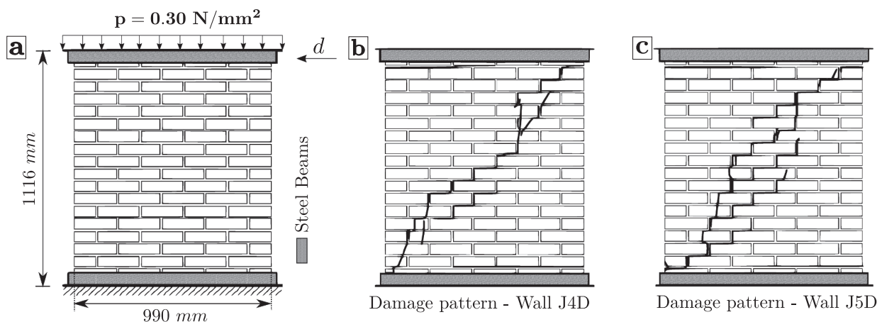
Fig. 5. (a) Schematic representation of solids clay brick masonry walls (J4D & J5D), loaded firstly by an overburden pressure of 0.30 N/mm 2 followed by a lateral prescribed displacement d ; and the experimental crack patterns of the walls (b) J4D and (c) J5D.
