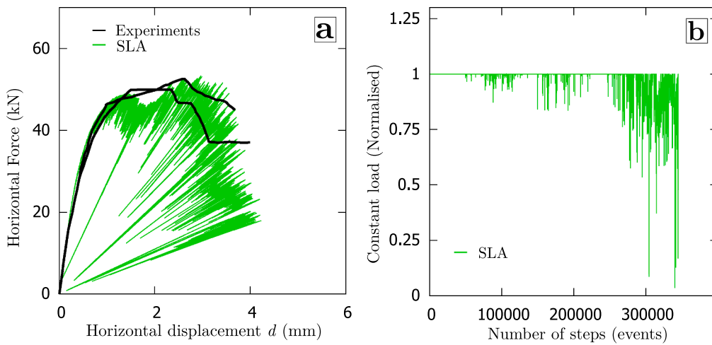
Fig. 17. Force–displacement curves of the experiments compared against those of the SLA for the 3D model, and (b) the evolution of constant load of precompression during the SLA simulation.
