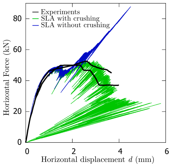
Fig. 10. Force-displacement curves of the SLA simulation of the micro models with and without crushing nonlinearities.
