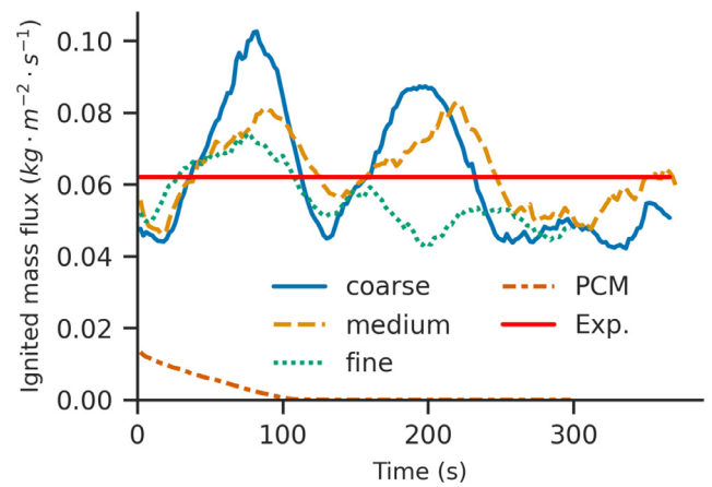
Fig. 4. Instantaneous ignited mass flux calculated using PCM and the proposed method with different grid resolution (data for Exp. is the mean ignited mass flux). The airflow rate is 0.276 kg \cdot m^{-2} \cdot s^{-1} , and the particle grid size is 1.5d_p .
