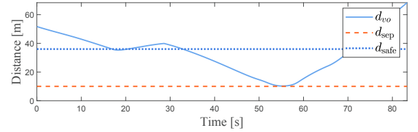
(b) Distance to the obstacle [m] during the simulation.
