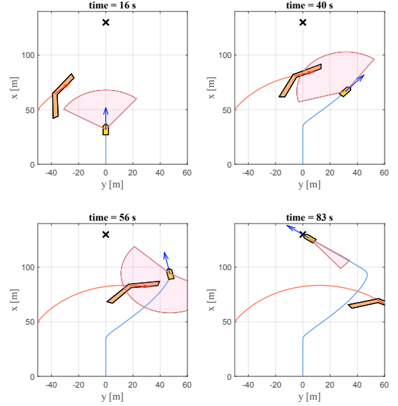
(a) North-East plots from the simulation. The vehicle and obstacle trajectories are given by the blue and red solid lines, respectively. The vehicle is the yellow polygon, and the obstacle is the orange polygon. The red, transparent sector represents the union of the sets \mathcal{E}(\mathbf{p}) along the obstacle boundary, with a radius of d_{\text{safe}} . The blue vector shows \psi_v , and the target position \mathbf{p}_t is marked by an 'X'.
