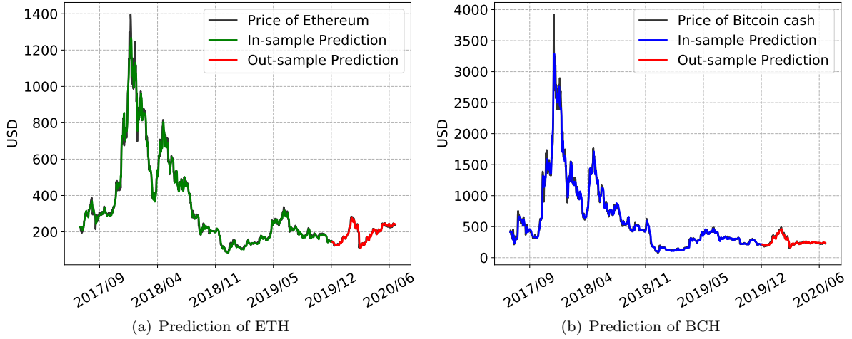
Figure 7: Prediction of the WAMC on ETH and BCH.
