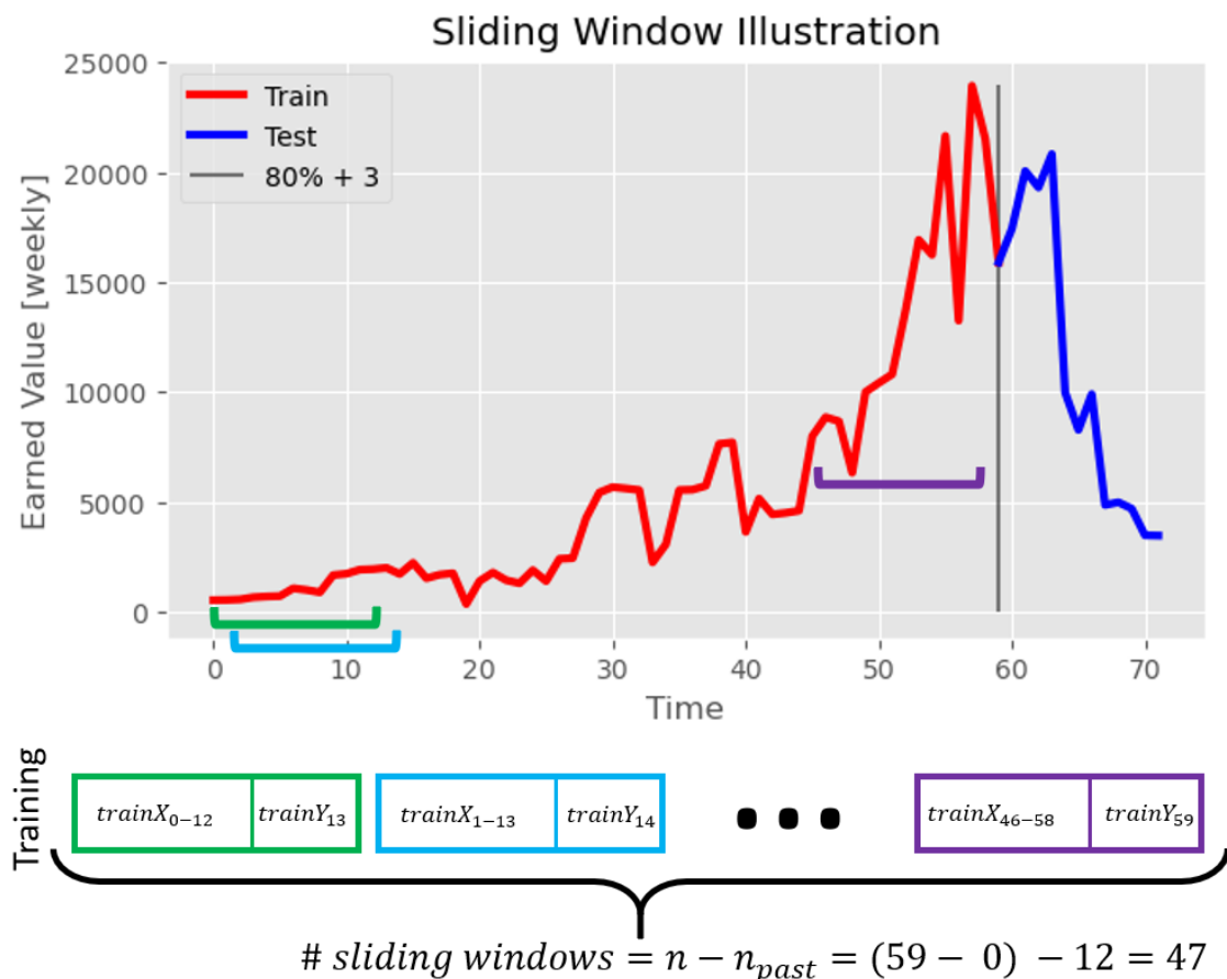
Figure 3.8: The figure present how the windows slides through the data.
