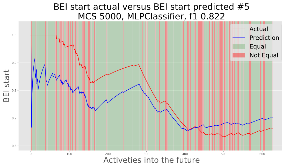
(a) MLPClassifier 1. Test 3.
