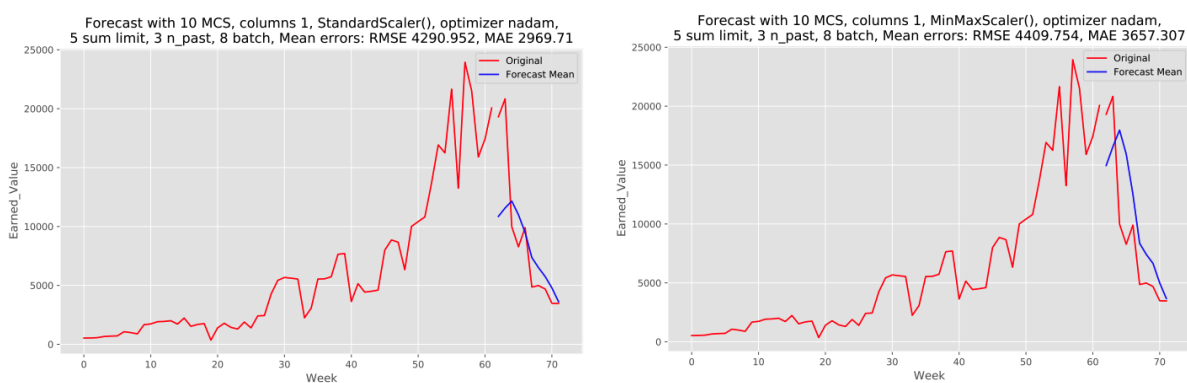
(a) Testing of the model with StandardScaler .
