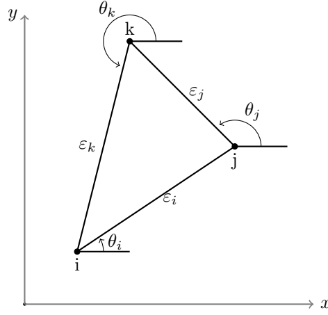
Figure 3.4.3: Triangle
