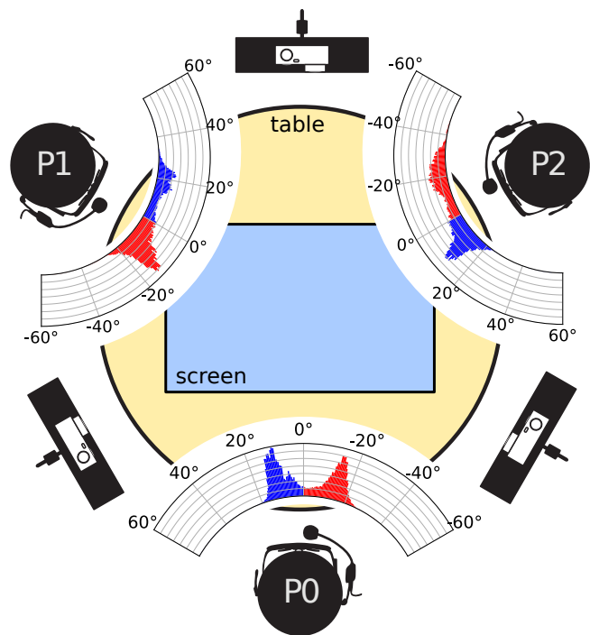
Fig. 2. Spatial configuration of the sensors and participants in the dataset. Each spoken interaction involves three participants seated at the positions denoted with P0, P1, and P2. The polar plots show the distribution of head rotations around the Y-axis (yaw) for each position, estimated over all sessions in the dataset. Angles are relative to the direction of the corresponding camera. Positive angles are plotted in blue and negative angles in red.
