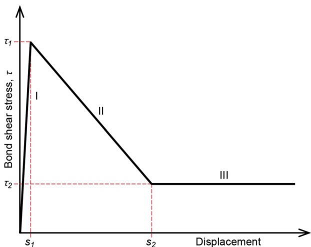
Fig. 2 Idealised trilinear bond slip model, based on Benmokrane et al. (1995)
