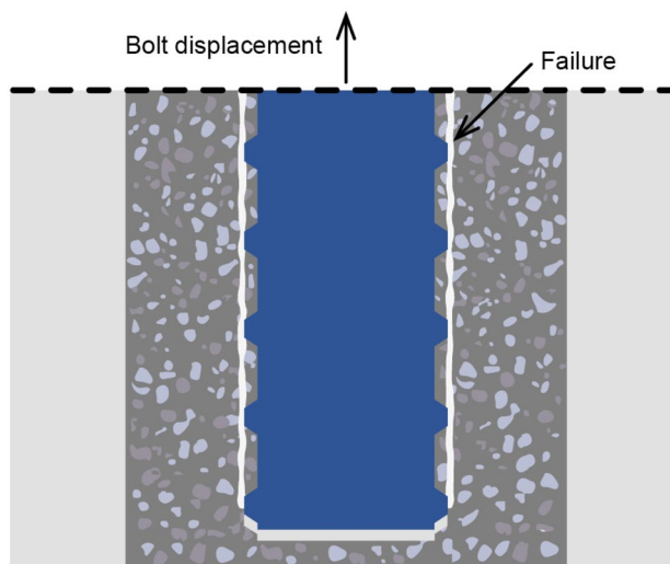
Fig. 4 Failure pattern of a rebar pull-out in the grout/bar-interface; redrawn based on Bigaj-van Vliet (1999) and Federation Internationale du Beton (2000)
