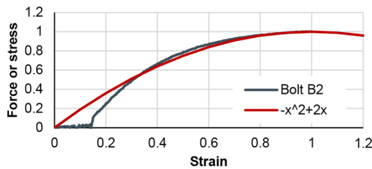
Fig. 10 Approximation of the stress–strain relationship
