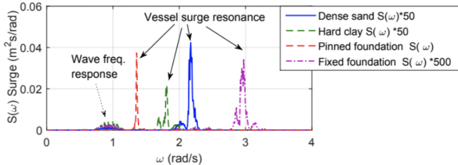
(b) Power spectra of the surge motion [112]
