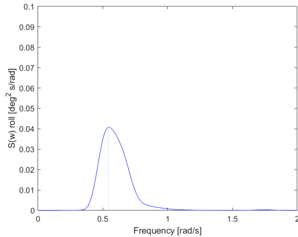
Figure 7.33: Power spectra of the SSCVs blade roll motion; head sea \theta_{wv} =270 deg; H_s= 1 m; T_p=7.3 s.
