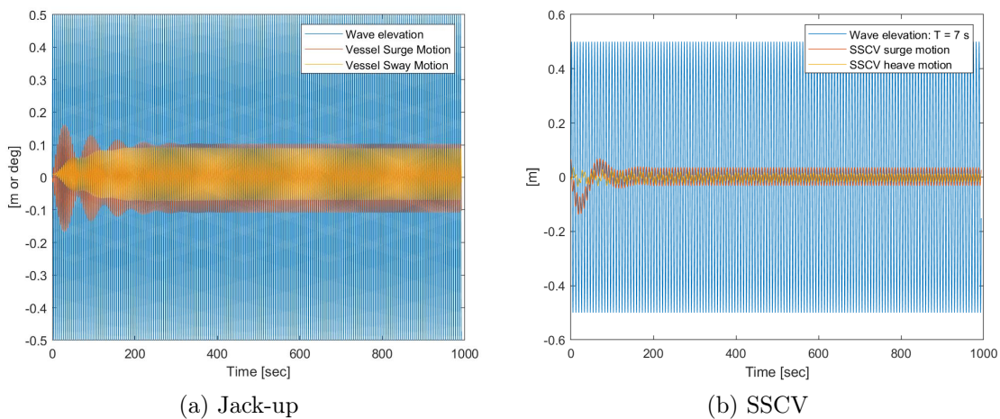
Figure 7.3: Time series for jack-up vessel and the SSCV showing the transient and the steady state period of the simulated time period.
