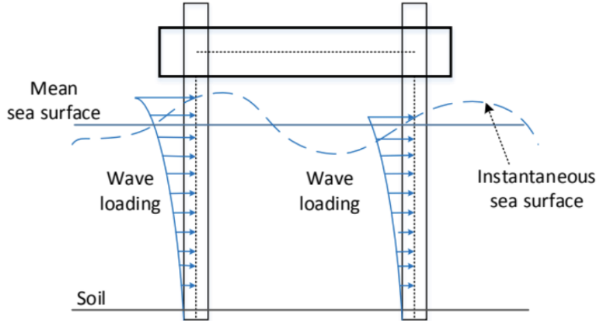
Figure 4.7: Wave loads acting on the jack-up legs. [6]
