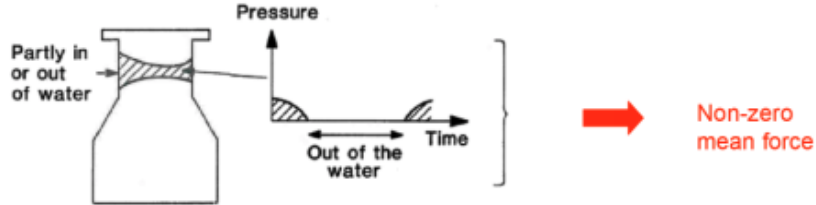
Figure 4.12: The mean value from second-order effects in variation of the wetted body surface. [22]
