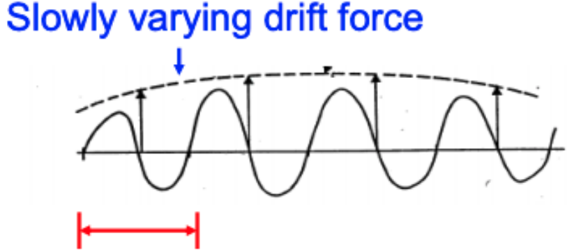
Figure 4.13: A slowly varying drift force. [22]
