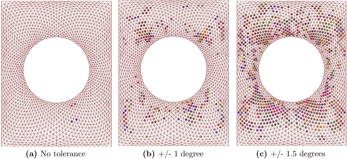
Figure 7.6: Similar node groups distribution for different angle tolerances.
