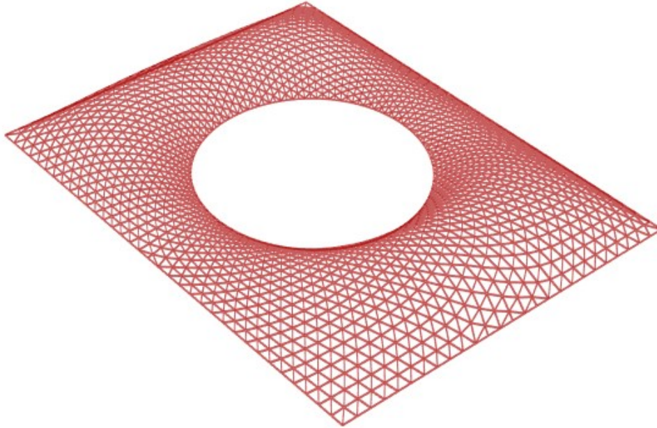
Figure 7.4: The original global shape and grid pattern of the Great Court Roof of the British Museum.
