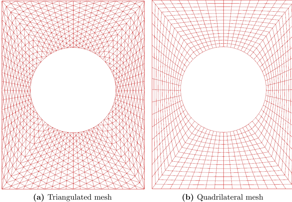
Figure 7.19: New mesh generated onto flat surface.
