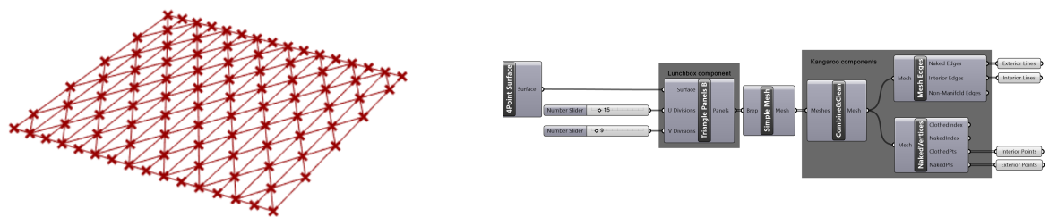
Figure 6.4: Convert one surface into a specific mesh. Triangle Panel B is from the LunchBox plugin. Combine&Clean , Mesh Edges and NakedVertices is from the Kangaroo plugin.
