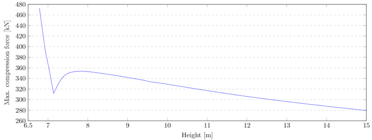
Figure 7.10: The maximum compression in the Great Court Roof depending on the global shape, which is differentiated by its height.
