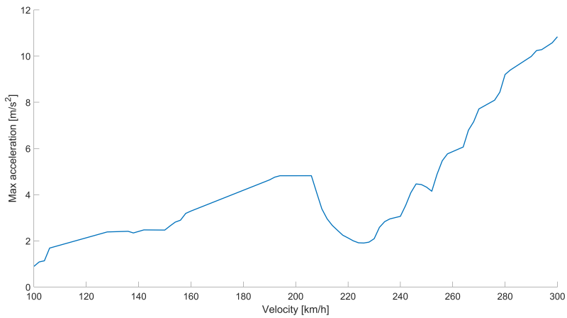
Figure 4.19: Envelope of all 10 HSLMA-trains for bridge number 401.
