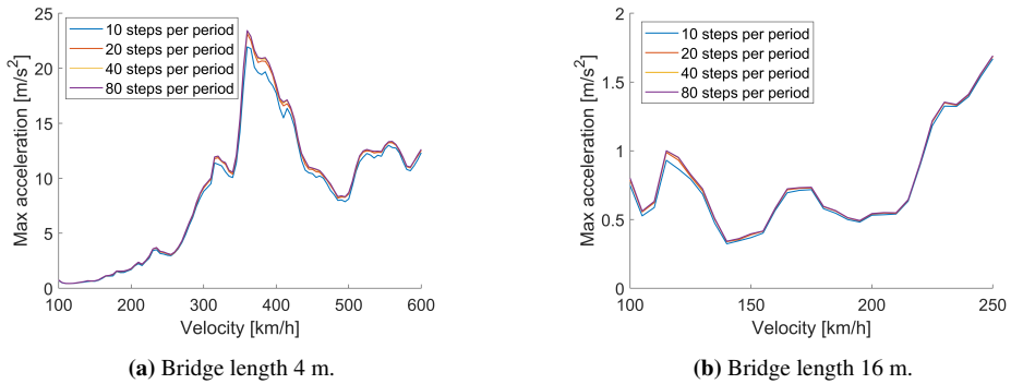
Figure 4.11: Velocity-Response calculated with 10, 20, 40 and 80 steps per period.
