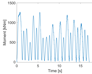
(b) IoE-calculation of moment from Train 2.
