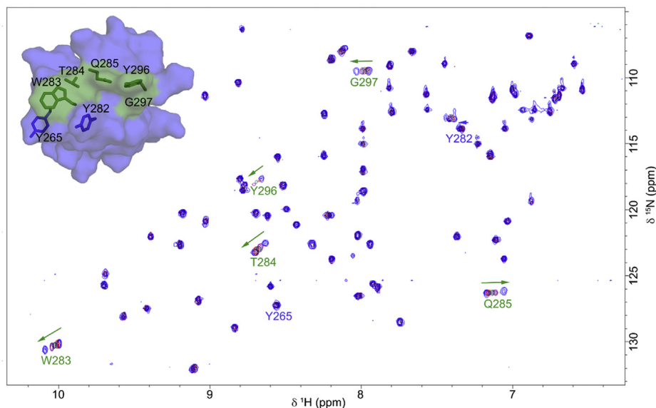
Figure 5. ^{15}\text{N} -HSQC of CjCBM5 interacting with (\text{GlcNAc})_6 . The figure shows an overlay of ^{15}\text{N} -HSQC spectra for CjCBM5 in the presence of (\text{GlcNAc})_6 at various concentrations (0.2, 1.0, 2.5, and 10 mM). The arrows indicate the direction of change in chemical shifts as a result of the titration of CjCBM5 with (\text{GlcNAc})_6 . Affected residues (W283, T284, Q285, Y296, and G297) are highlighted in green on the surface model of CjCBM5 . Other surface-exposed aromatic residues for which no significant chemical shift perturbation was detected (Y265 and Y282) are shown in blue for illustration purposes. HSQC, heteronuclear single quantum coherence.
