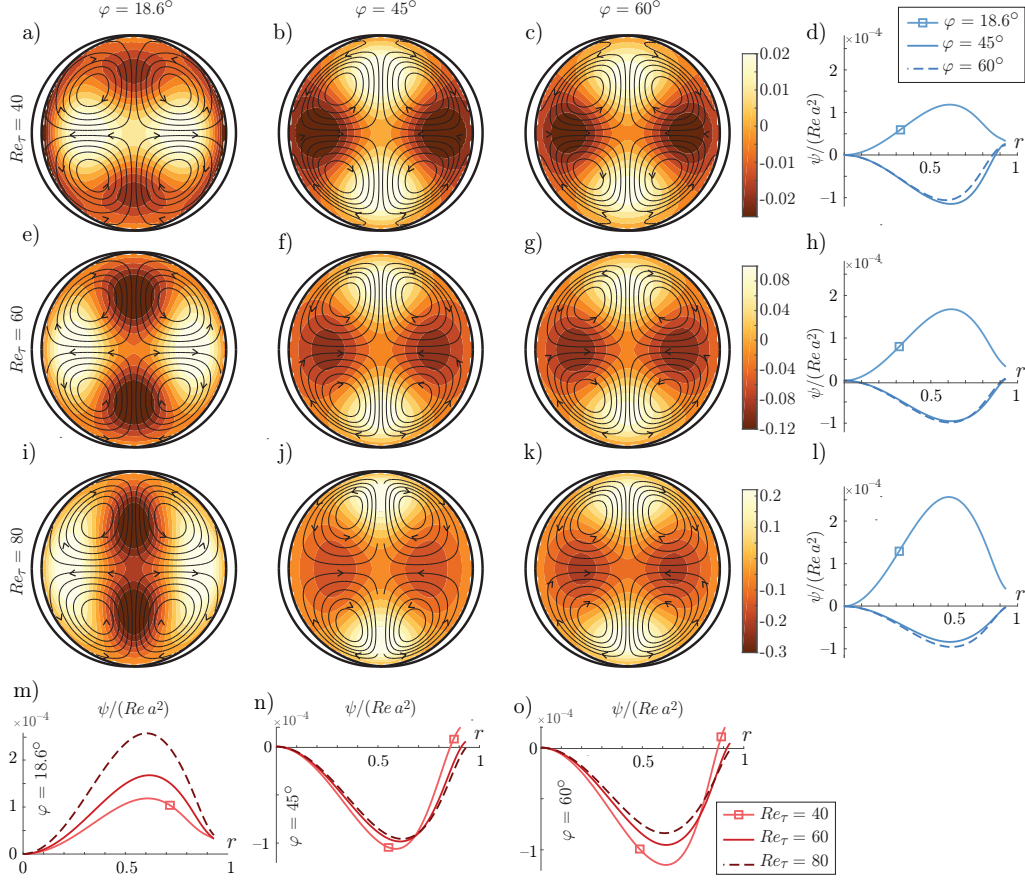
FIGURE 3. Simulation results, a = 0.05, \kappa = \pi and m = 1 . Re_\tau is the same along the first three rows, and \varphi is the same along the first three columns, as indicated. (a-c,e-g,i-k): Black curves are contours of \psi/(Re a^2) indicating streamlines, arrows indicate flow direction; colour contours show deviation of \bar{u}_{z,\text{tot}} from Poiseuille flow as defined in equation (4.5). (d,h,l,m-o): plots of \psi/(Re a^2) along the ray \theta = \pi/4 . A common legend applies to all plots where \varphi varies at constant Re_\tau (d,h,l), and vice versa (m-o).
