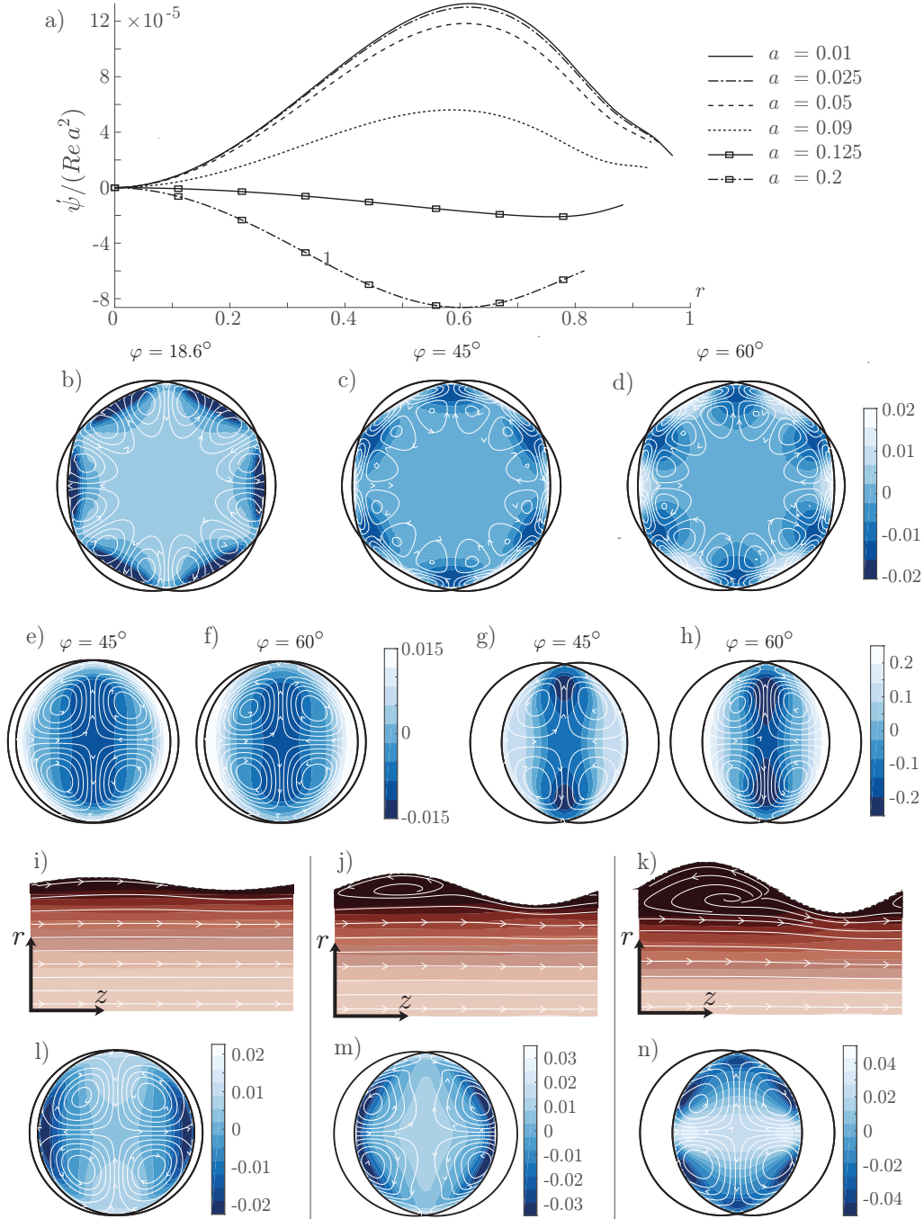
FIGURE 4. Simulation results. (a) Scaled circulation strength along \theta = \pi/4m_1 for \varphi = 18.6^\circ , m_1 = 1 and increasing a ; graphs from top to bottom: a = 0.01, 0.025, 0.05, 0.09, 0.125, 0.2 . Panels (b-h, l-n): streamwise-averaged flow (streamlines) and pressure (colour contours, average pressure subtracted). Panels (b-d): m_1 = 3 , all other panels m_1 = 1 . Crossing angle \varphi = 18.6^\circ except as indicated. Amplitudes are a = 0.05 (b-f, i, l), a = 0.125 (j, m), a = 0.2 (g, h, k, n). (i-k): streamlines in a streamwise section of the pipe through crests/troughs at \theta = \pi/2 , lighter (darker) colour indicates higher (lower) average absolute velocity.
