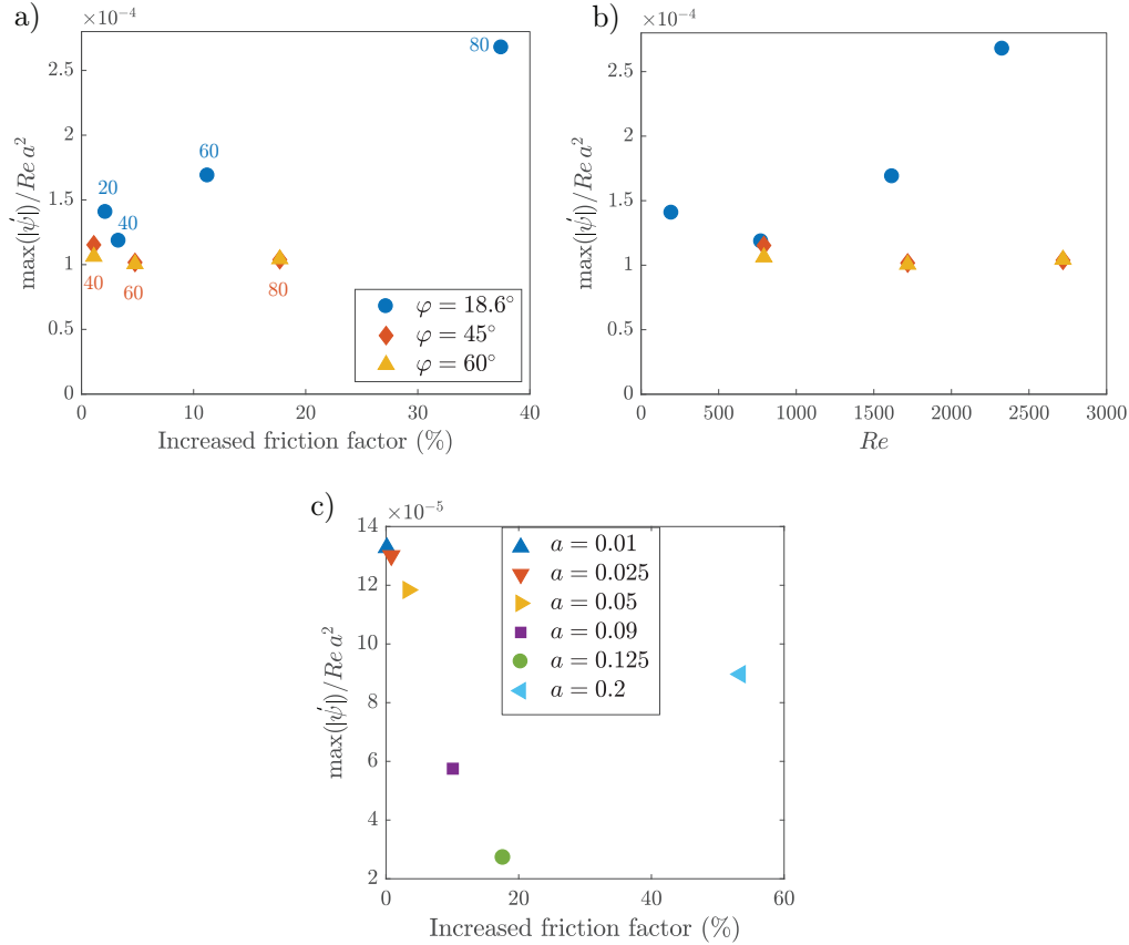
FIGURE 5. Maximum circulation strength plotted against increase in friction factor (i.e., increased head loss) in percent. a) Comparison of three different crossing angles for m = 1 , a = 0.05 — corresponding values of Re_\tau are indicated for each marker (common for overlapping markers); b) same cases as in panel a, but with Reynolds number as abscissa; c) increasing amplitude for Re_\tau = 40 and m = 1 .
