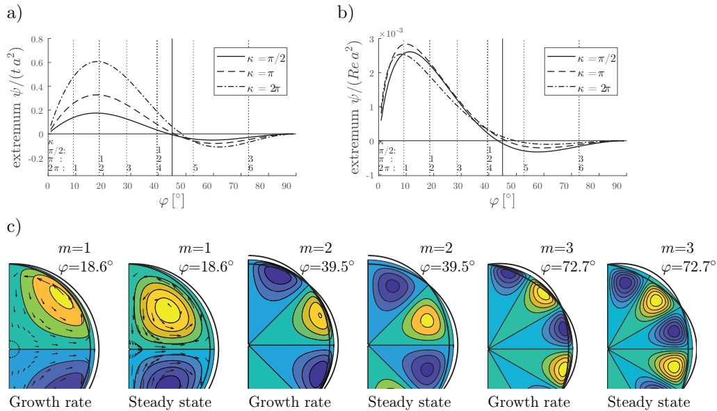
FIGURE 9. Initial growth rate compared to final steady-state solution. a) Initial growth rate, inviscid, b) Ultimate, steady-state solution, c) streamlines.
