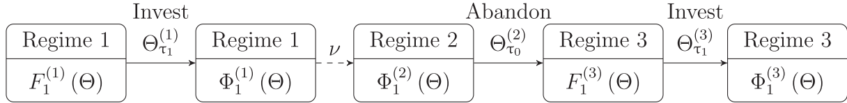
Fig. 1. State-transition diagram.
