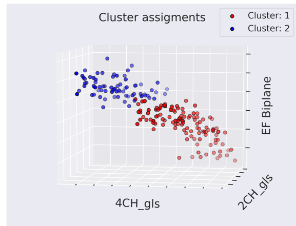
(b) Ward/2 cluster assignments.
