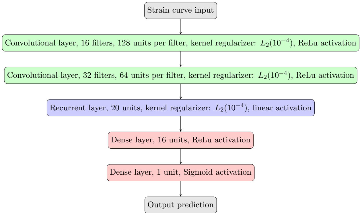
Figure 6.3: A block diagram illustrating the architecture of the ANN used in this work.
