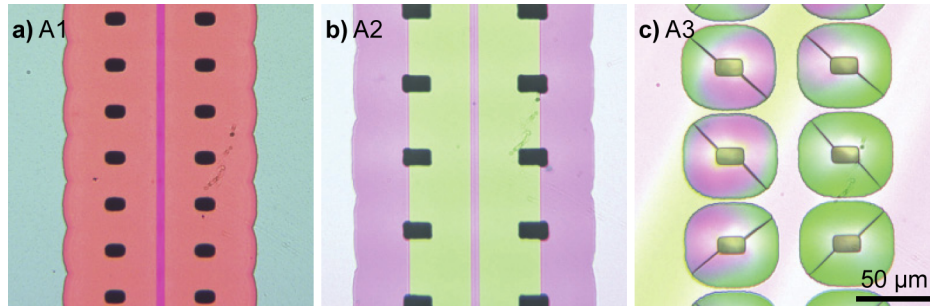
Fig. 6. Optical microscope images of the fabricated membranes. a) Sample A1 under-etched in XeF 2 with SiO 2 and Al 2 O 3 layer stack for passivation. b) Sample A2 under-etched in SF 6 plasma after the TMAH treatment, which removed the SiO 2 /Al 2 O 3 layer stack. The shallow etching, which defines the waveguides, only extends to the openings. c) Sample A3 also under-etched in SF 6 plasma. The scale bar in (c) applies to all images.
