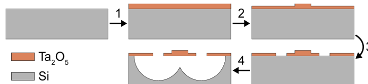
Fig. 3. Process flow for fabrication of suspended waveguides. Film deposition (1) is followed by consecutive patterning of waveguides (2) and etching openings (3). In the final step, the waveguide is under-etched (4).
