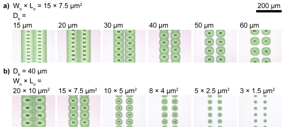
Fig. 7. Result of under-etching test in SF 6 plasma after 30 min with lateral spacing 2 \times D_a = 60 \mu\text{m} between openings. a) Effect of different longitudinal spacings of the etching openings with dimensions 15 \times 7.5 \mu\text{m}^2 ( W_o \times L_o ). b) Effect of different openings sizes with a constant longitudinal spacing D_b = 40 \mu\text{m} .
