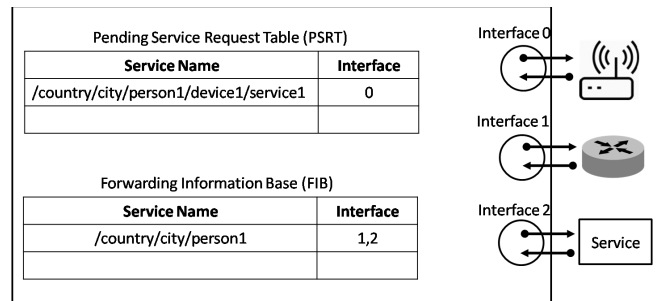
Fig. 3: Forwarding table of a NDN node.
