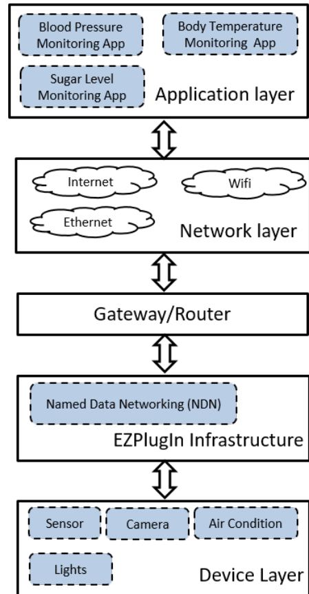
Fig. 1: Architecture of EZPlugIn framework for smart home.
