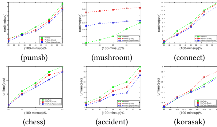
Fig. 6. Runtime of the PrePost+ with and without the CBPM framework.
