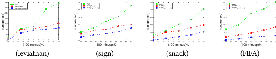
Fig. 10. Runtime of the FAST with and without the CBPM framework.
