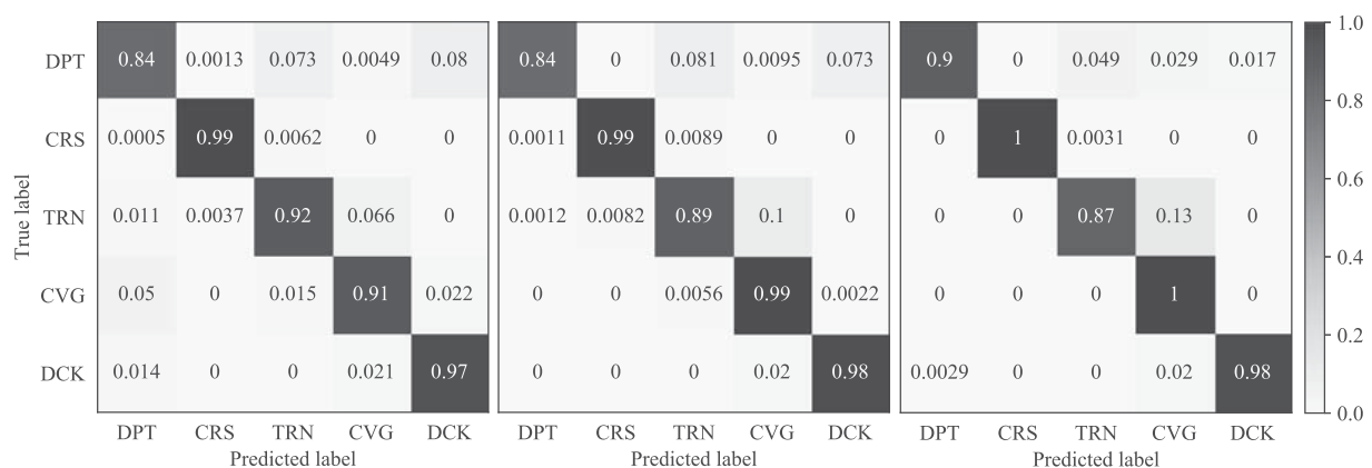
Figure 6. Confusion matrix reflecting precision by scenarios (left: CLF No.4; middle: CLF No. 9; right: CLF No. 14). (This figure is available in colour online.)
