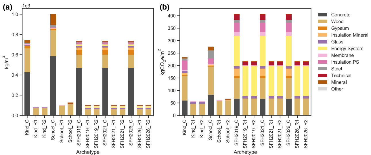
FIGURE 3 (a) Material intensity per m^2 per archetype; (b) emission intensities per m^2 per archetype. Underlying data used to create this figure can be found in Supporting Information S2
