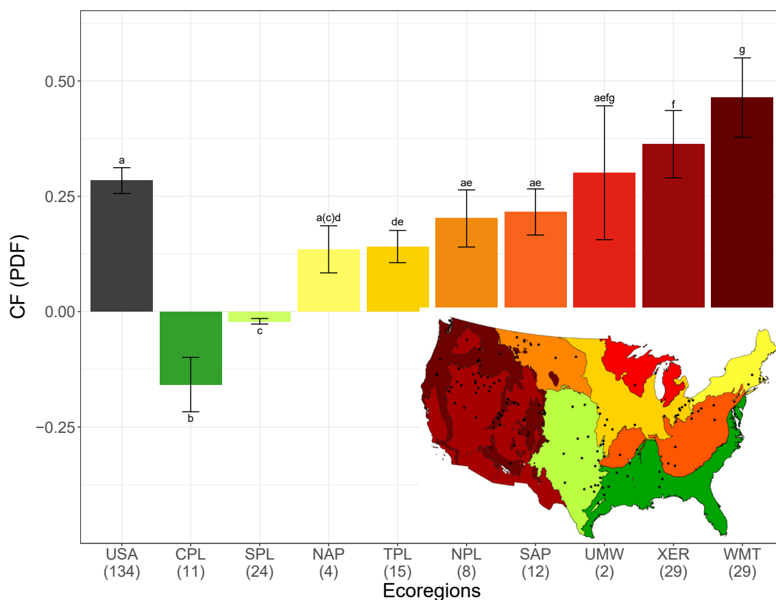
Figure 2. Barplot showing a mean characterization factor (CF) in Potentially Disappeared Fraction of species (PDF \pm 95% confidence interval; CI) at the United States (USA) level ( PDF_{usa} shown in dark grey) and at the ecoregion level ( PDF_{eco} color coded, with ecoregions as a gradient of intensity). We used letters to identify which PDF_{eco} differed or not from each other. When two bars share a letter, they are not significantly different from each other and marginally not significantly different from each other when the letter is in parentheses. A positive PDF represents a loss of taxa, whereas a negative
