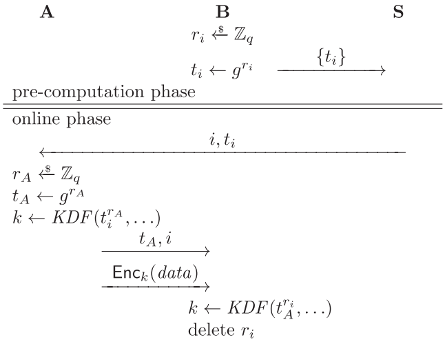
FIGURE 4. Key exchange with pre-computed keys.
