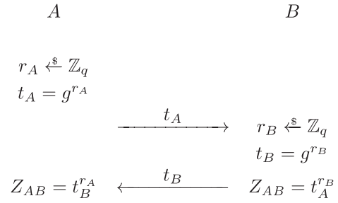
FIGURE 2. Diffie–Hellman key agreement. A protocol with forward secrecy.
