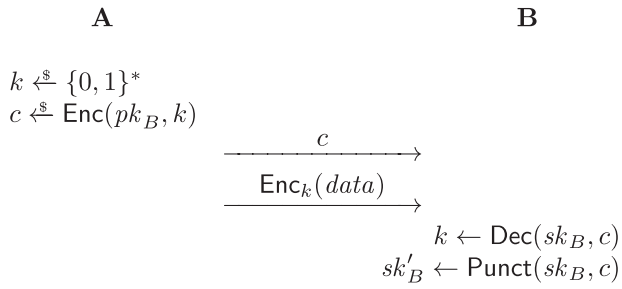
FIGURE 3. Key exchange from puncturable encryption.
