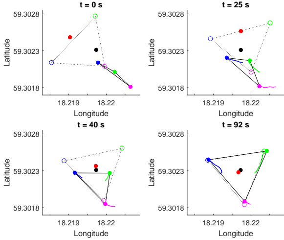
Fig. 9. Experimental result showing how the agent formation converges to the desired distances while the estimated target position goes towards the actual. The ducklings (blue, green and magenta dots) start in almost collinear positions with the target (black), which gives a bad estimated target position (red). Desired agent positions (circles) are calculated from the current positions. As time increases the actual agents converge to a better formation and the estimation error decreases. Four steps of the process are shown.
