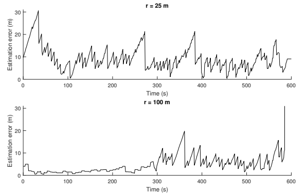
Fig. 13. Plot of the error of the estimated target position for two additional test runs, with the radius of the desired formation at 25 and 100 meters respectively.
