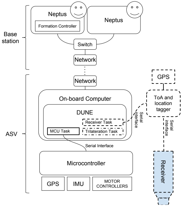
Fig. 4. Overview of the system during operation. Dashed lines denote subsystems and processes used only in agents. The dot-dash line denote the trilateration process running in the target.
