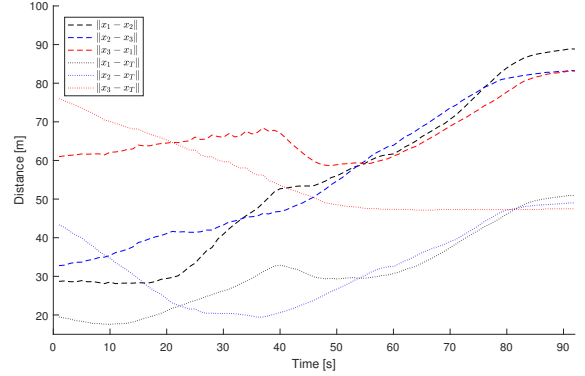
Fig. 10. Plot of the errors of the formation when converging to surround the target. The distance between the ASVs and the actual position of the target goes to toward the set distance of r = 50 meters while the distances between each ASV goes towards d_{i,j} = d = \sqrt{3}r .
