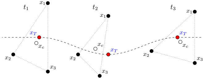
Fig. 1. Illustration of how the three agent formation tracks the target moving along a trajectory. The agents x_i , i = 1, 2, 3 , with the centroid x_c , are given over three time steps together with the target estimations x_T in red. By the agents forming the desired formation \Phi , and where the centroid attempts to align with the target estimation, the system is able to acquire sufficient localization ability to keep tracking the target.
