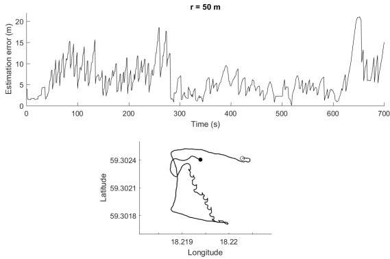
Fig. 12. Plot of the error between the actual and estimated target position over 700 seconds with a desired formation with 50 m radius. The path of the target in the lower figure. Initial and final positions as circle and dot respectively.
