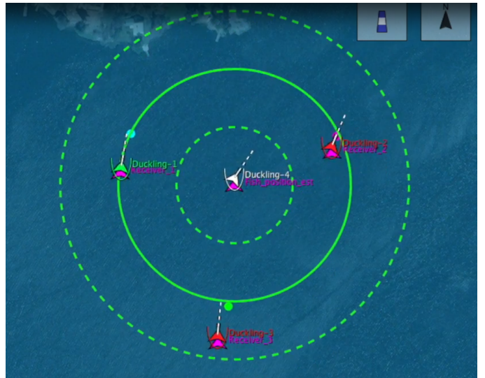
Fig. 8. Partial screen capture of the interface in Neptus during execution of the experiment. The coloured dots are current values of x_i while the arrows are actual positions x_{i,N} of the ASVs with attached receivers. The full green circle is the current radii of \Phi , i.e. the desired distance from agent to target.
