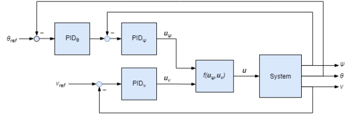
Fig. 5. Block diagram of the low-level control used by the ducklings. \theta_{ref} is the absolute bearing towards the coordinate \mathbf{x} , \theta the current bearing and \psi the yaw rate. \mathbf{u} is the combined inputs to the thrusters used both for yaw and forward propulsion v .
