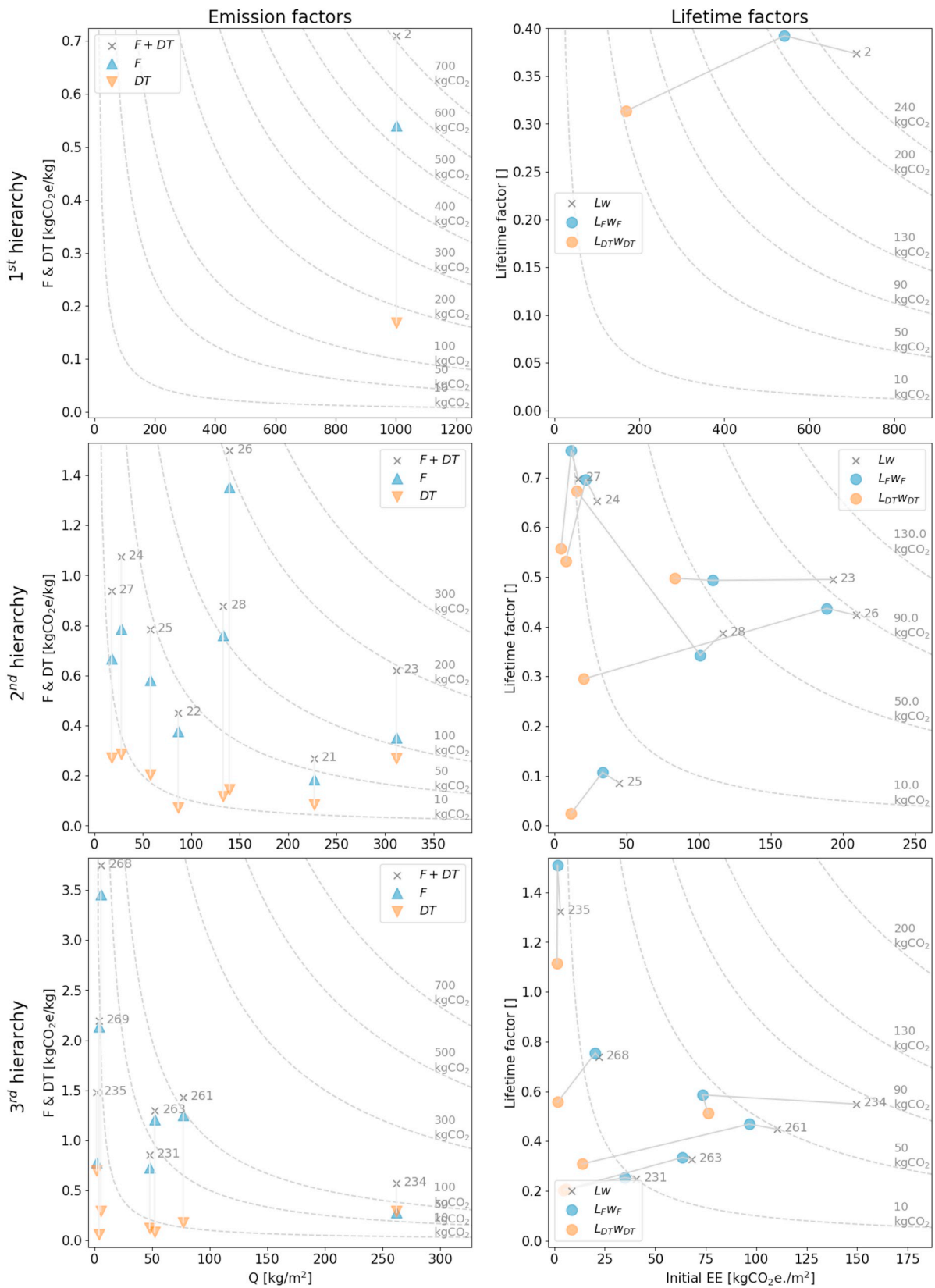
Fig. 6. The Q - F - DT plots in the left column show the EE in \text{kgCO}_2\text{e./m}^2 of the initial lifecycle phases broken down by quantities and emission factors. The EE - L_F - L_{DT} plots in the right column show the EE of the replacement lifecycle phases broken down by initial EE and lifetime factors. The dashed contour lines are the products of the horizontal and vertical axes and show the resulting EE. The plots show results from building element '2 Envelope, foundations, and structure' from the case building at the 1st, 2nd, and 3rd hierarchies, where BE are numbered according to NS3451. Building element names for the numbering can be found in Fig. 4.
