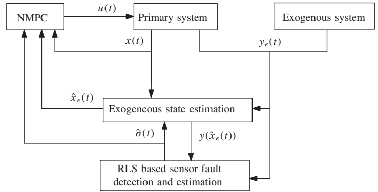
FIGURE 1 Illustration of proposed FTNMPC scheme.
