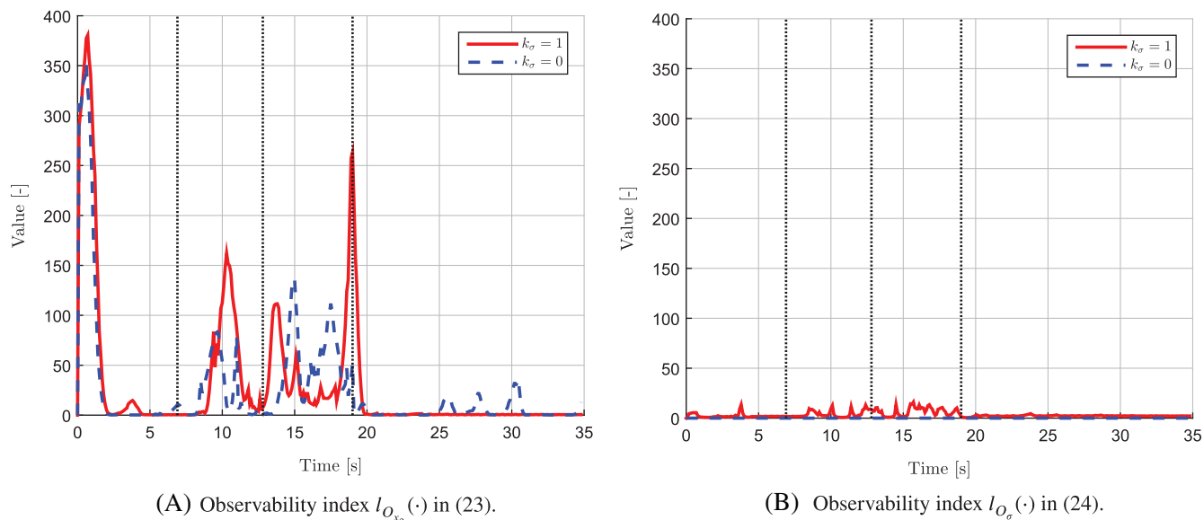
FIGURE 5 Time series of the two decomposed observability indices in (22) for the exogenous state for different values of k_\sigma . Saturation (limit) value for l_{O_{x_e}}(\cdot) is \frac{k_{x_e}}{\epsilon_1} = 10^6 , while for l_{O_\sigma}(\cdot) the value is \frac{k_\sigma}{\epsilon_2} = 10^5 . Black dotted vertical lines indicate onset of incipient bearing fault at t=7 s, complete bearing fault at t=13 s, and healthy bearing and onset of slowly developing range fault at t=19 s. Note that l_{O_\sigma}(\cdot) \equiv 0 for the blue dashed line with k_\sigma=0 . [Colour figure can be viewed at wileyonlinelibrary.com ]
