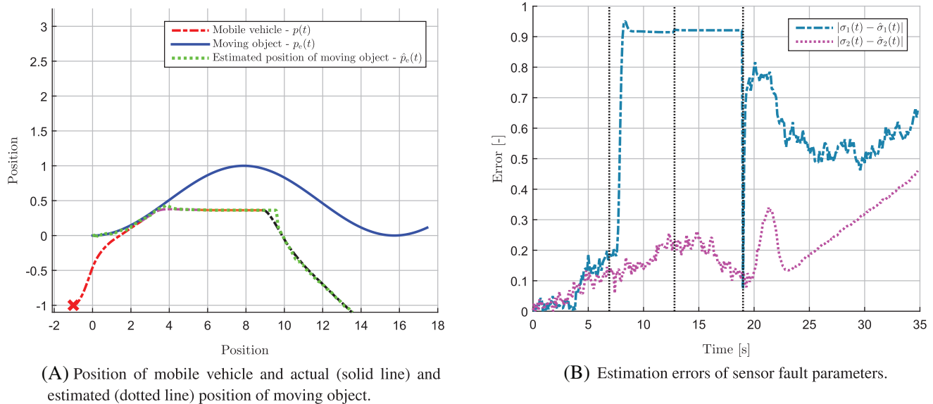
FIGURE 3 Simulation results with no observability indices in the objective function (13) of the NMPC controller, showing, A, positions of the mobile vehicle and moving object and B, estimation errors of the sensor fault parameters. [Colour figure can be viewed at wileyonlinelibrary.com ]
