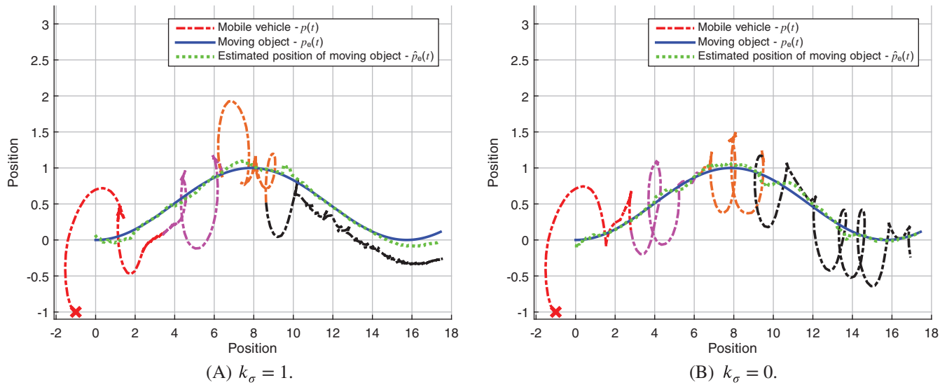
FIGURE 2 The position of the mobile vehicle, and the actual and estimated position of the moving object. The position of the mobile vehicle is shown with a red dotted line before the onset of the bearing fault, with a purple line during the partial bearing fault, an orange line during the complete bearing fault, and with a black line during the range fault [Colour figure can be viewed at wileyonlinelibrary.com ]
