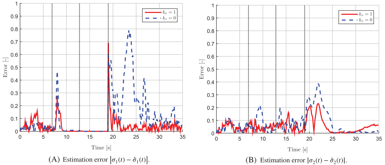
FIGURE 4 Estimation errors (absolute values) for the sensor fault-parameters \sigma(t) for simulations with k_\sigma=1 and k_\sigma=0 . Black dotted vertical lines indicate onset of the incipient bearing fault at t=7 s, complete bearing fault at t=13 s, and healthy bearing and slowly developing range fault at t=19 s. [Colour figure can be viewed at wileyonlinelibrary.com]
