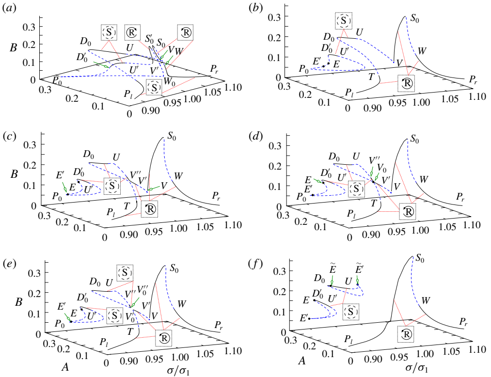
FIGURE 12. The same as in figures 10 and 11 but for \gamma = \pi/12 . The semi-axis ratio \delta_1 = 0.0 in (a) (harmonic oblique reciprocity), \delta_1 = 0.6 (b), \delta_1 = 0.743 (c), \delta_1 = 0.744 (d), \delta_1 = 0.745 (e) and \delta_1 = 0.9 (f). The physical input data are taken from (3.30). The panels qualitatively repeat the wave-amplitude metamorphoses of the response curves in figures 10 and 11. An exception is the branch D'_0U'P_0D'_0 , which does not emerge from a single point as happened for \gamma = \pi/6 . The latter fact implies two (not one) stable nearly standing wave modes (points on D_0U and D'_0U' ) existing for all 0 \leq \delta_1 \leq 1 .
