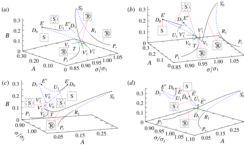
FIGURE 9. The metamorphosis of the steady-state wave-amplitude response curves for the diagonal-type ( \gamma = \pi/4 ) counterclockwise elliptic forcing with \delta_1 equal to: (a) 0.75, (b) 0.785, (c) 0.786 and (d) 0.95. The physical input parameters are defined in (3.30). Notation and symbols are taken from figure 8. Comparing the panel (a) with figure 8(b) indicates the vanishing stability ‘island’ U_1'U_1 (nearly standing waves) and appearance of the ‘island’ V_1'V_1'' (stable counterclockwise swirling). Zone of irregular waves does not increase. Panels (b) and (c) show an emerge of one from two loop-type branches, which are expected in the limit \delta_1 \rightarrow 1 . For \delta_1 = 0.785 in (b), the ‘island’ V_1'V_1'' touches TD_0 to constitute bifurcation point V_0 . A further increase of \delta_1 (panel (c), \delta_1 = 0.786 in computations) divides the branching at this bifurcation point and leads to the continuous response curve P_1TV_0'V_1'S_0R_1P_r (counterclockwise swirling) and the loop-type branch D_1E''U_1E'D_0V_0'D_1 (the nearly standing sloshing except at E'' where a (purely) standing wave is expected). Panel (d) shows that the branching becomes close to that in figure 4 as \delta_1 tends to the unit (the circular tank orbit).
