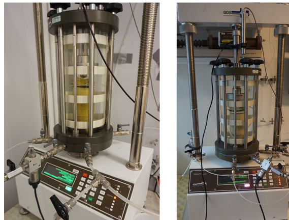
Figure A.10. The two sets of GDSLab triaxial testing equipment used.
