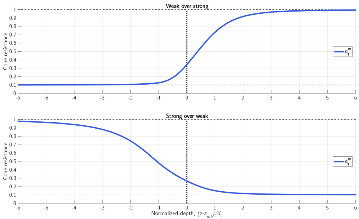
Figure B.9. Presentation of cone resistance with normalized depth along the x -axis. The interface is presented with a vertical line. Dotted lines on top of 1 and at the bottom of 0.1 represents the strong and weak cone resistances, respectively.
