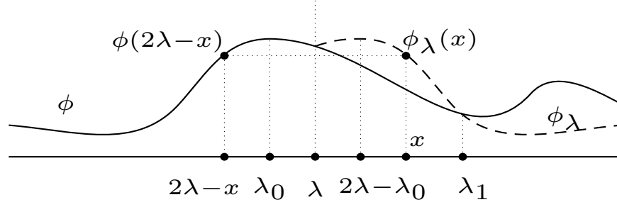
FIGURE 1. Assume that the procedure of pushing x = \lambda from left to right stops for the first time at a local maximum of \phi at x = \lambda_0 . Then, the reflection axis x = \lambda is pushed slightly to the right side of x = \lambda_0 , which generates a non-empty set \Sigma_\lambda^- denoted by the interval (\lambda, \lambda_1) . \phi_\lambda as the reflection of \phi is partially depicted by dashed lines. For a point x \in \Sigma_\lambda^- , its reflection 2\lambda - x is also depicted.
