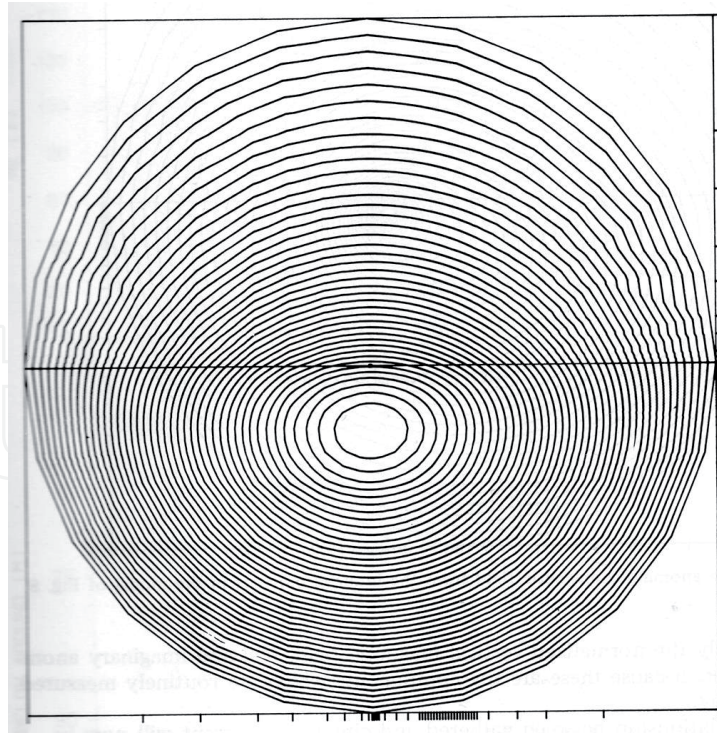
Figure 2. Secondary magnetic field from induced currents in a conducting half-space [6].
