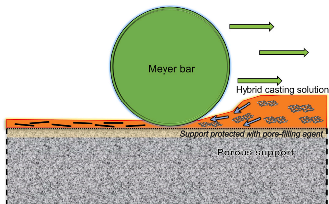
Fig. 7. Schematic illustration of orientation of GO-based fillers in hybrid membranes fabricated using bar coating technique.
