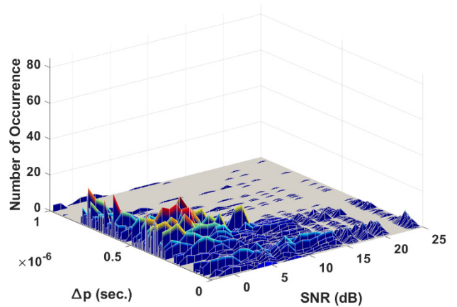
FIGURE 8. Effect of SNR on the transient start detection performance of PD method.
