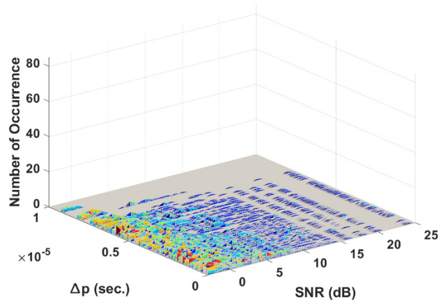
FIGURE 5. Effect of SNR on the transient start detection performance of BSCD method.
