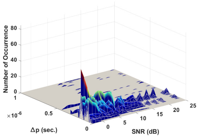
FIGURE 9. Effect of SNR on the transient start detection performance of EC-∅ method.
