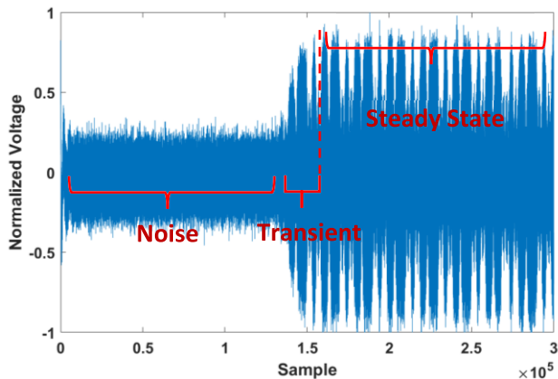
FIGURE 2. A sample recording from Wi-Fi signals captured in the laboratory.
