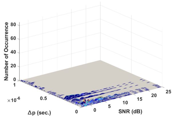
FIGURE 10. Effect of SNR on the transient start detection performance of EC- \alpha method ( \theta = 30 ).
