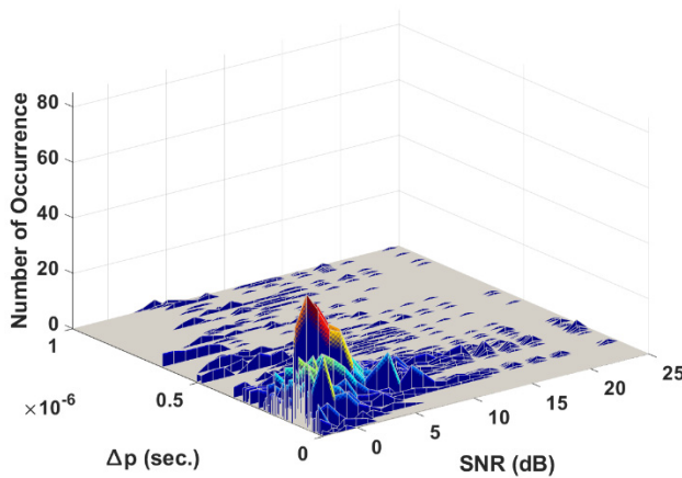
FIGURE 7. Effect of SNR on the transient start detection performance of MCPD method.
