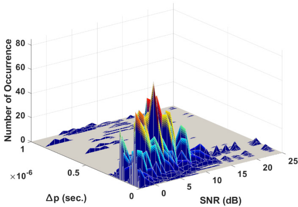
FIGURE 6. Effect of SNR on the transient start detection performance of VFDTD method.
