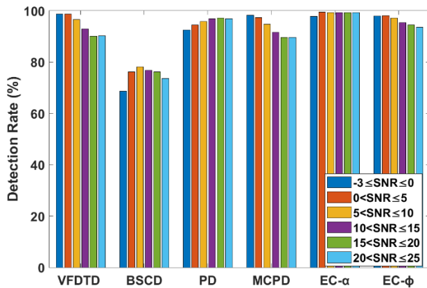
FIGURE 11. Effect of SNR on the transient start detection performance of EC- a method.
