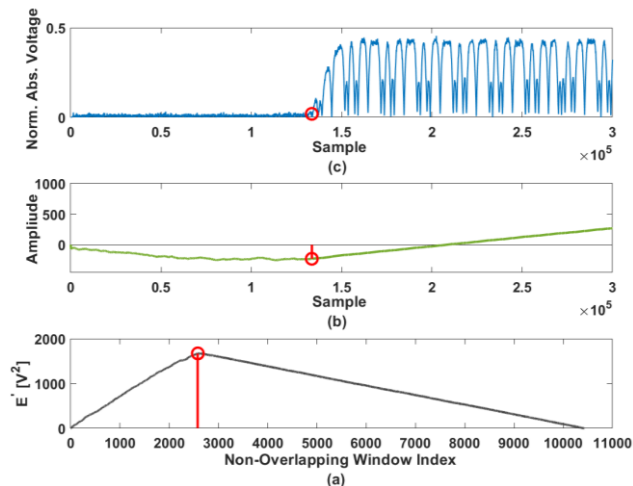
FIGURE 4. (a) The energy curve obtained by using EC- \emptyset method, (b) The unwrapped instantaneous phase signal, (c) The detected transient starting point.
