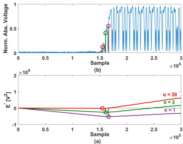
FIGURE 3. (a) The energy curve obtained by using EC- \alpha method, (b) The detected transient starting points.
