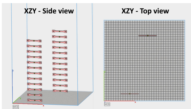
Fig. 13 Schematic representation of specimens' placement in the build chamber in XZY orientation for one run (Magics 20.0)
