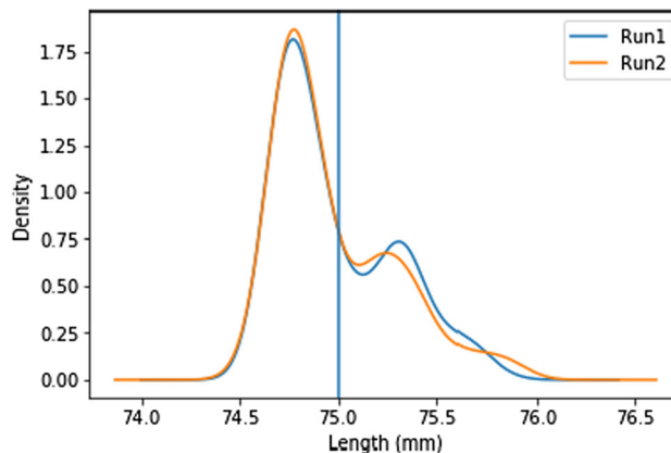
Fig. 6 Distribution of measured length for run 1 and run 2 based on kernel density estimation (The nominal value is 75 mm)
