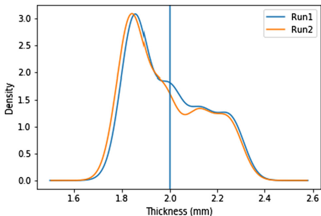
Fig. 4 Distribution of measured thickness for run 1 and run 2 based on kernel density estimation (The nominal value is 2 mm)
