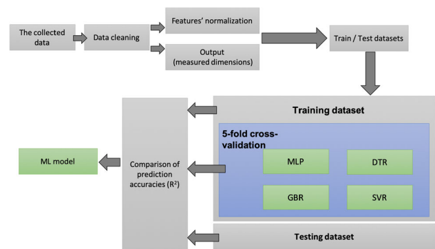
Fig. 10 Representation of data analysis pipeline
