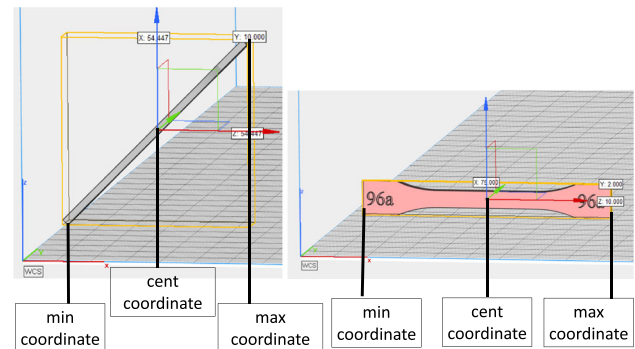
Fig. 11 Example of part placement description in the build chamber through maximal, central and minimal coordinates for Angle and XZY orientation using Magics 20.0
