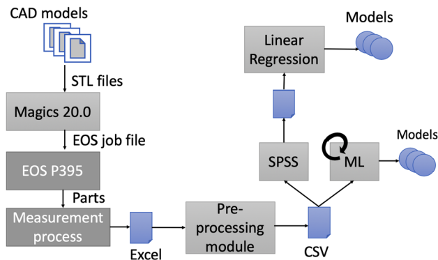
Fig. 2 The schematic representation of the process from build layout design to predicted models
