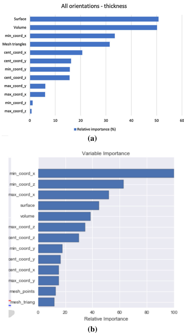
Fig. 26 Predicted significance of the parameters on thickness: a Pearson correlation test results, b Gradient boost regressor
