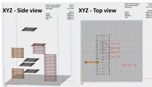
Fig. 12 Representation of specimens' placement in the build chamber in XYZ orientation for one run (Magics 20.0)
