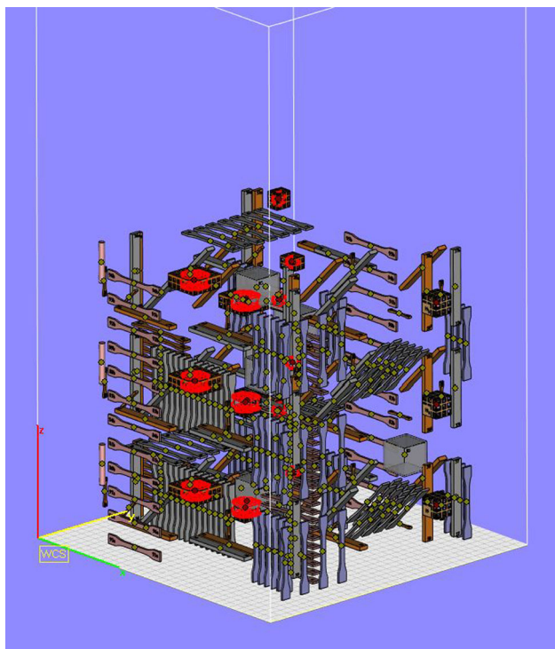
Fig. 1 Build layout in Magics 20.0
