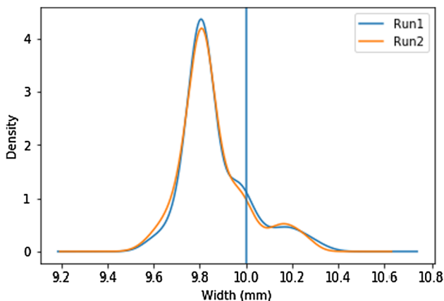
Fig. 5 Distribution of measured width for run 1 and run 2 based on kernel density estimation (The nominal value is 10 mm)
