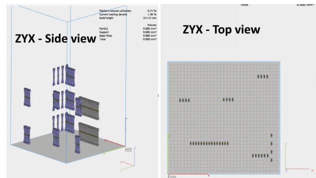
Fig. 14 Representation of specimens' placement in the build chamber in ZYX orientation for one run (Magics 20.0)
