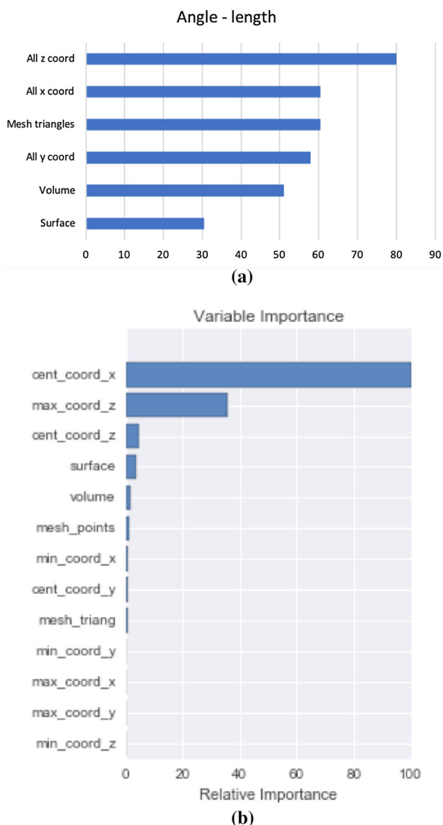
Fig. 19 Significance of parameters for length in Angle orientation: a Pearson correlation test results, b Decision Tree regression results
