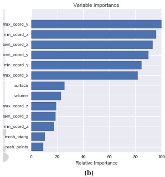
Fig. 17 Significance of parameters for width in XZY orientation: a Pearson correlation test results, b Gradient boosting regression results
