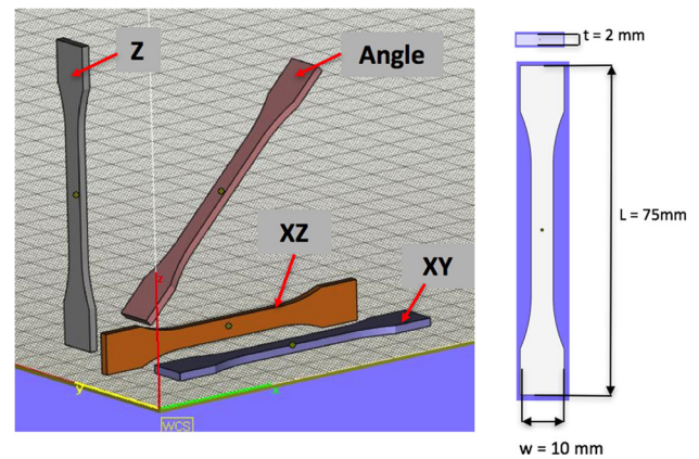
Fig. 3 Schematic visualization of parts' orientation and dimensional features (where t —thickness, w —width and L —length )
