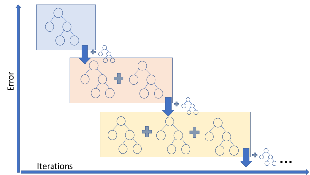
Fig. 8 Schematic representation of gradient boosting regression in regards to algorithm iterations
