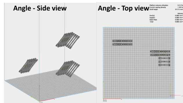
Fig. 15 Representation of specimens' placement in the build chamber in Angle orientation for one run (Magics 20.0)
