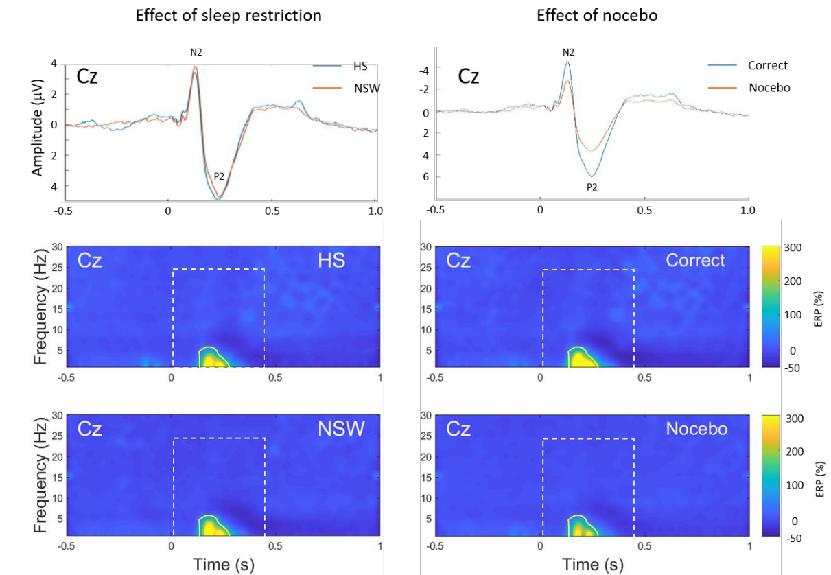
Figure 1. Top: Time-domain average from electrode Cz with the effect of sleep restriction (left) and nocebo (right). Bottom: Time-frequency domain grand average from electrode Cz with the effect of sleep condition and nocebo. White dashed rectangle indicates 1–400 ms / 1–25 Hz search area. Yellow line indicates exact region of interest. HS: Habitual sleep. NSW: Night shift work.
