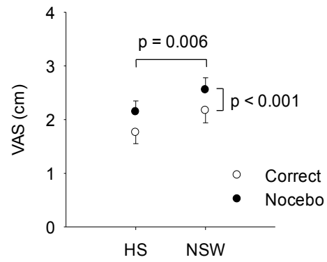
Figure 2. Electrical pain by sleep and nocebo conditions. There was a main effect of sleep ( p = 0.006 ), and a main effect of nocebo ( p < 0.001 ), but no sleep x nocebo interaction ( p = 0.6 ). Values are estimated marginal means.
