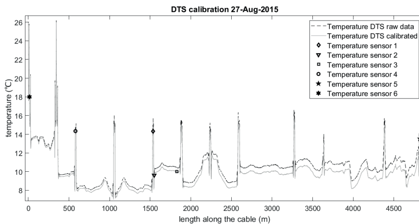
Figure 4. DTS calibration by six standard thermometers along the installed fiber-optic cable.
