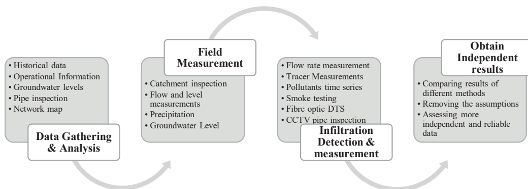
Figure 3.1 Systematic method for detecting unwanted water in the sewer system (Beheshti, Sægrov and Ugarelli, 2015).
