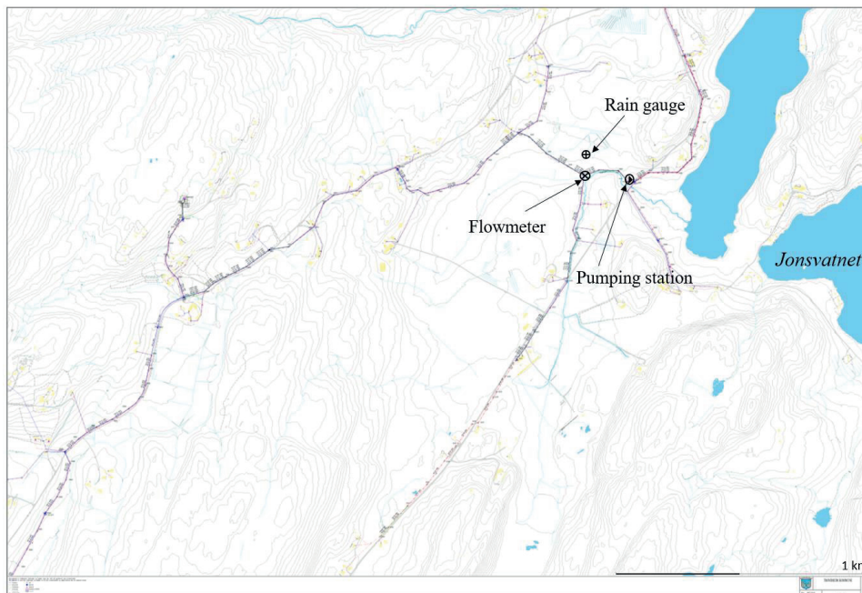
Figure 4.2 Wastewater network in Lykkjebekken catchment with location of rain gauge, flowmeter, and pumping station (Trondheim Municipality, 2013).
