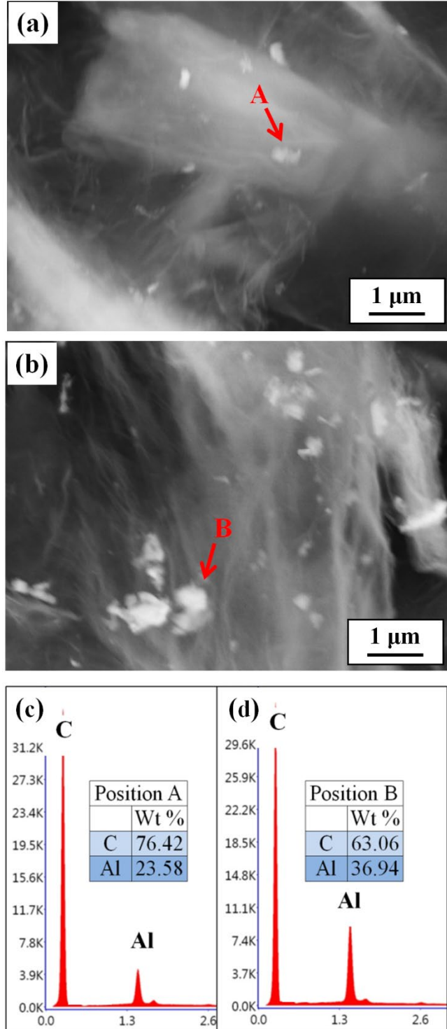
Fig. 3 SEM microstructures of Al-coated graphene with a reaction time of (a) 0.5, (b) 1.0 h; (c) and (d) EDS spectra of the corresponding sample.
