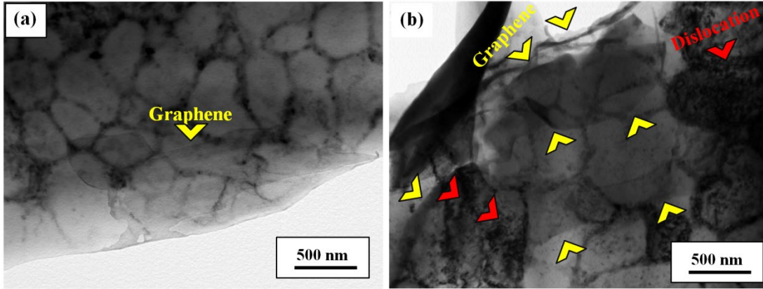
Fig.17 TEM microstructures of graphene/ AlSi10Mg composites prepared by SLM: (a) before deformation, (b) after deformation.
