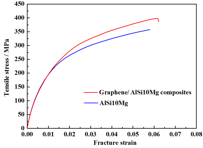
Fig. 13 Engineering stress-strain curves for AlSi10Mg alloy and graphene/ AlSi10Mg composites.
