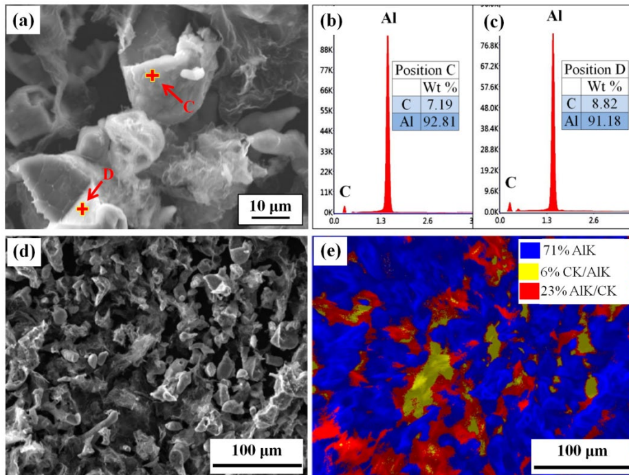
Fig. 5 SEM microstructures of (a, d) Al-coated graphene, (b, c) composition analysis at point C and D, (e) Al and C distribution maps of Al-coated graphene. The coating time was 1.5 hrs.
