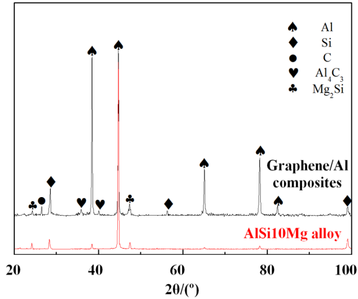
Fig. 10 XRD patterns for Al-coated graphene reinforced AlSi10Mg nanocomposites.
