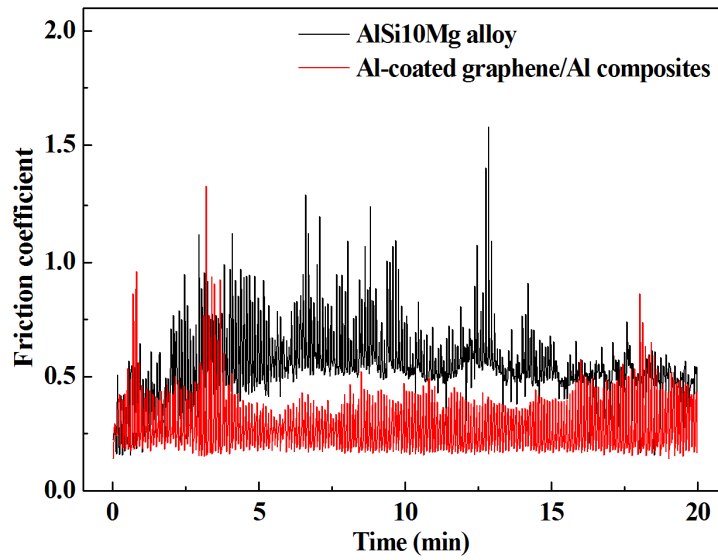
Fig. 14 The curve of friction coefficient and time.
