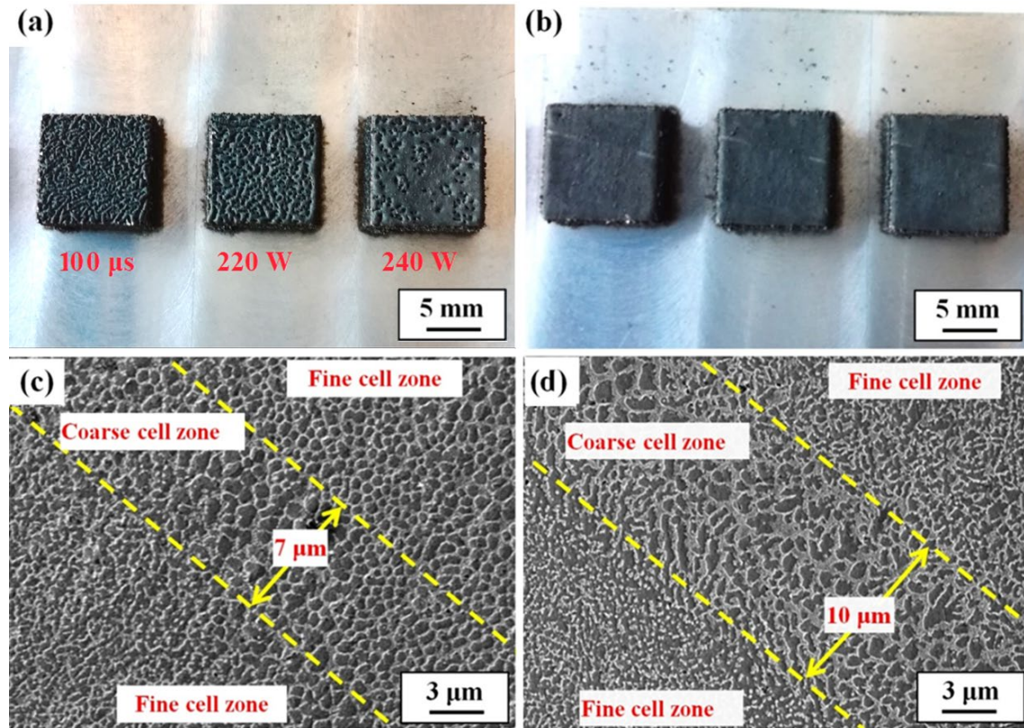
Fig. 9 Al-coated graphene/AlSi10Mg composites prepared by SLM different exposure time (100 \mu s) and laser power (220W, 240W) (a), Al-coated graphene/AlSi10Mg composites prepared by SLM exposure time 140 \mu s and laser power 300 W(b), the microstructure of Al-coated graphene/AlSi10Mg composites (cross section) prepared by SLM (c), the microstructure of AlSi10Mg alloy (cross section) prepared by SLM (d).
