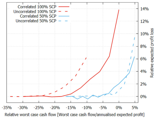
Fig. 4. The efficient frontiers for the different versions of the large instance. Let E^* be the annualized expected profit without cash flow control, and E^{\bar{F}} the annualized expected profit using cash flow threshold \bar{F} . The vertical axis represents the ratio 100 * (E^* - E^{\bar{F}}) / E^* . Let WC^{\bar{F}} be the worst-case cash flow obtained for a given threshold \bar{F} . The horizontal axis represents the ratio 100 * WC^{\bar{F}} / E^* . Finally, SCP is an abbreviation for space charter price.
