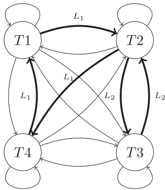
Fig. 2. Graph representation of an example network with four trades and two loops.
