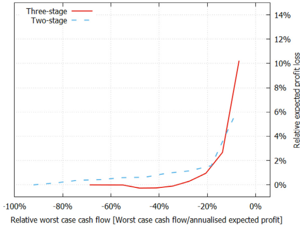
Fig. 7. The efficient frontiers for the three and two stage solutions for the small instance with uncorrelated correlation random variables and reduced space charter price. Let E^* be the annualized expected profit without cash flow control, and E^{\bar{F}} the annualized expected profit using cash flow threshold \bar{F} . The vertical axis represents the ratio 100 * (E^* - E^{\bar{F}})/E^* . Let WC^{\bar{F}} be the worst-case cash flow obtained for a given threshold \bar{F} . The horizontal axis represents the ratio 100 * WC^{\bar{F}}/E^* .
