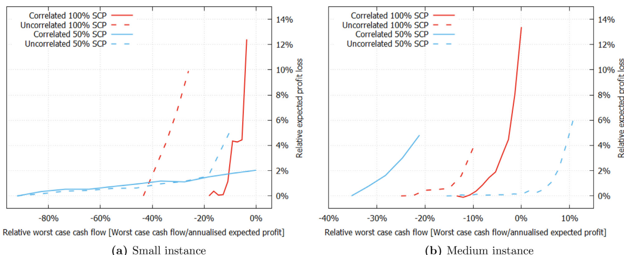
Fig. 5. The efficient frontiers for the different versions of the small and medium instances. Let E^* be the annualized expected profit without cash flow control, and E^{\bar{F}} the annualized expected profit using cash flow threshold \bar{F} . The vertical axis represents the ratio 100 * (E^* - E^{\bar{F}})/E^* . Let WC^{\bar{F}} be the worst-case cash flow obtained for a given threshold \bar{F} . The horizontal axis represents the ratio 100 * WC^{\bar{F}}/E^* . Finally, SCP is an abbreviation for space charter price.
