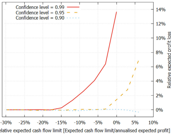
Fig. 6. The efficient frontiers for the CVaR model solved for the large instance with correlated random variables and normal space charter price. Let E^* be the annualized expected profit without cash flow control, and E^{\bar{F}_c} the annualized expected profit using cash flow threshold \bar{F}_c . The vertical axis represents the ratio 100 * (E^* - E^{\bar{F}_c})/E^* . The relative expected cash flow limit is calculated as the minimum expected cash flow allowed, \bar{F}_c , divided by the annualized expected profit.
