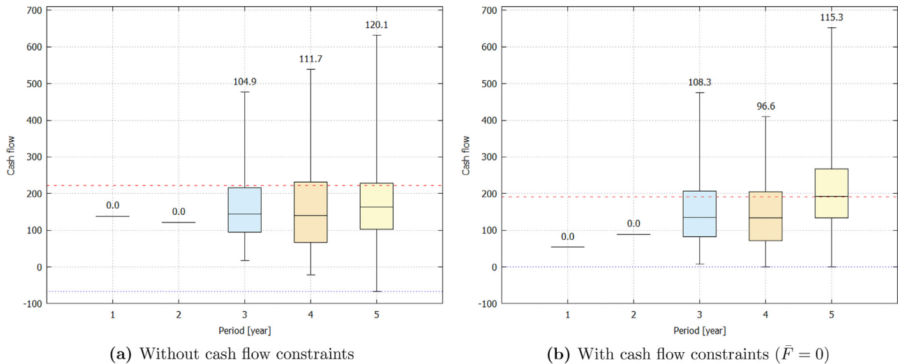
Fig. 3. The cash flow development for the large instance with correlated random variables and normal space charter price. The red dashed line is the annualized expected profit, and the numbers above each whisker is the standard deviation for the given period. (For interpretation of the references to colour in this figure legend, the reader is referred to the web version of this article.)
