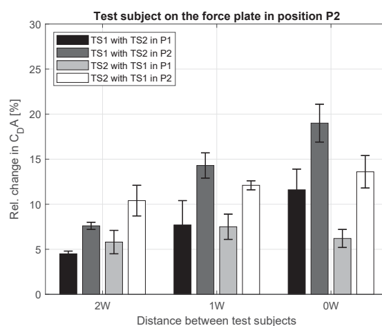
Fig. 7 Change in drag, relative to individual measurements, for two test subjects side-by-side. (a) shows the test subject on force plate in P1 and (b) in P2. The error bars are indicating the standard deviation with n=3
