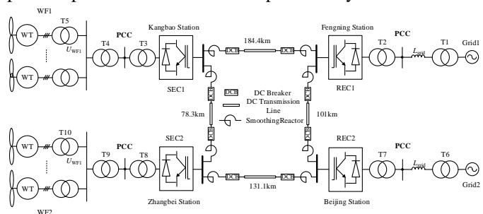
Fig. 1. An MTDC system with wind farm and synchronous AC grid integration.
