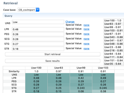
Fig. 4. A Query and its retrieval result in the myCBR workbench
