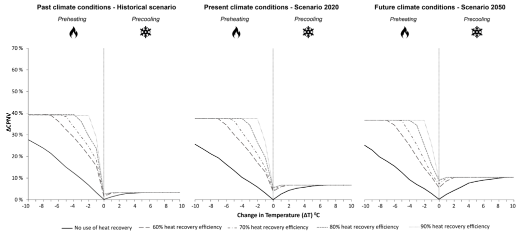
FIG. 24 Graph showing \Delta CPNV, with different efficiency for heat recovery system along with preheating and precooling in Milan for historical, 2020 and 2050 scenarios
