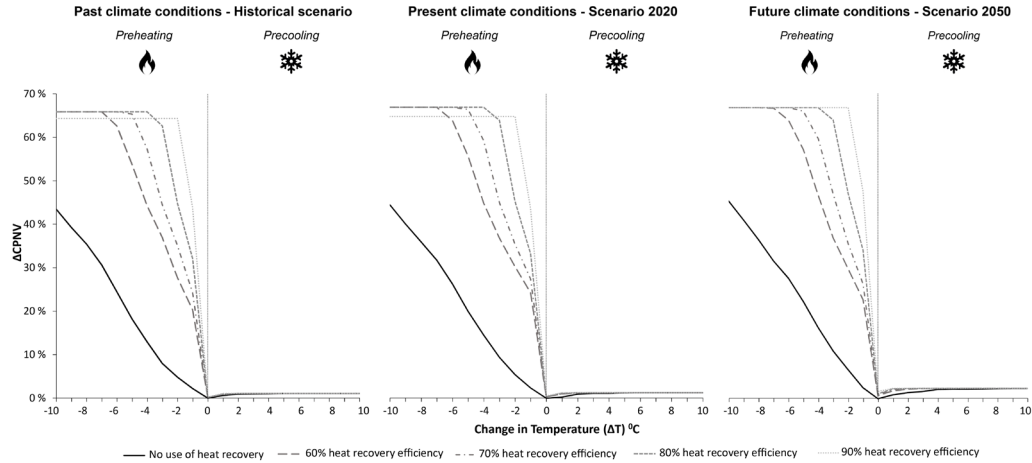
FIG. 23 Graph showing \Delta CPNV, with different efficiency for heat recovery system along with preheating and precooling in Brussels for historical, 2020 and 2050 scenarios
