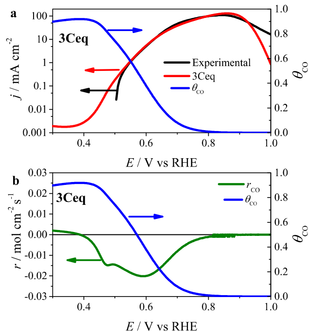
Figure 5: Comparison of the relative rates and the change in CO coverage, a) shows the total rate = v_1 + 3v_{\text{CO}} + v_{\text{OH}} + v_{\text{CO}_2} + v_{\text{PtO}} compared with the 3Ceq result and the CO coverage, \theta_{\text{CO}} , b) shows the net CO rate, r_{\text{CO}} = v_1 - v_{\text{COOH}} , compared with the CO coverage, \theta_{\text{CO}} .
