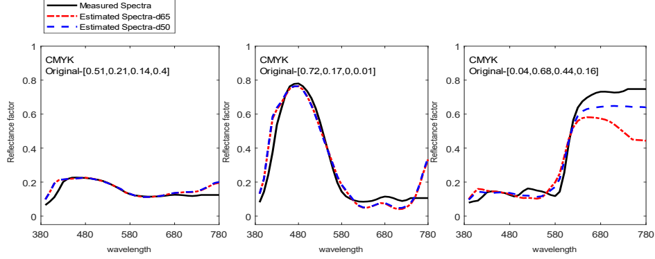
Fig. 4. Estimated reflectances of FOGRA51 using weighted PCA and 3135 training set: 5 th , 50 th and 95 th percentile RMS errors.
