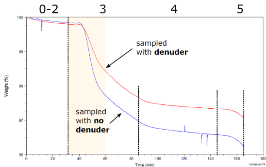
Figure 15. Normalized mass loss from TGA during devolatilization.
