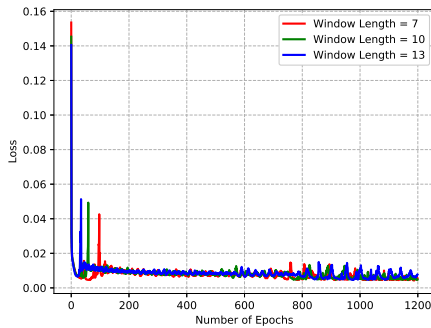
Fig. 12: The loss of LSTM-Attention-CNN Model with different window length of input size
