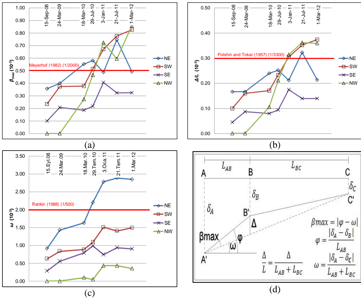
Fig. 8: Calculated wall distortions: (a) angular distortion, (b) deflection ratio and (c) rigid rotations
