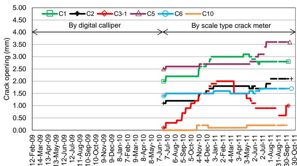
Fig. 6: Opening and closures of the pre-existing localized cracks
