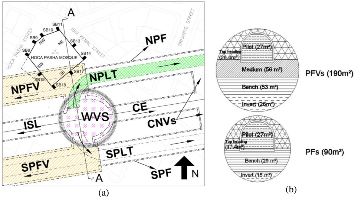
Fig. 2: (a) Location and neighbouring excavation works (b) Tunnel cross-sections (modified from Method Statements for Excavation and Support Works, 2008).
