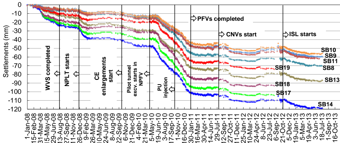
Fig. 4: The settlement time-history of the mosque (modified from Monthly Monitoring Reports, 2008-2013)
