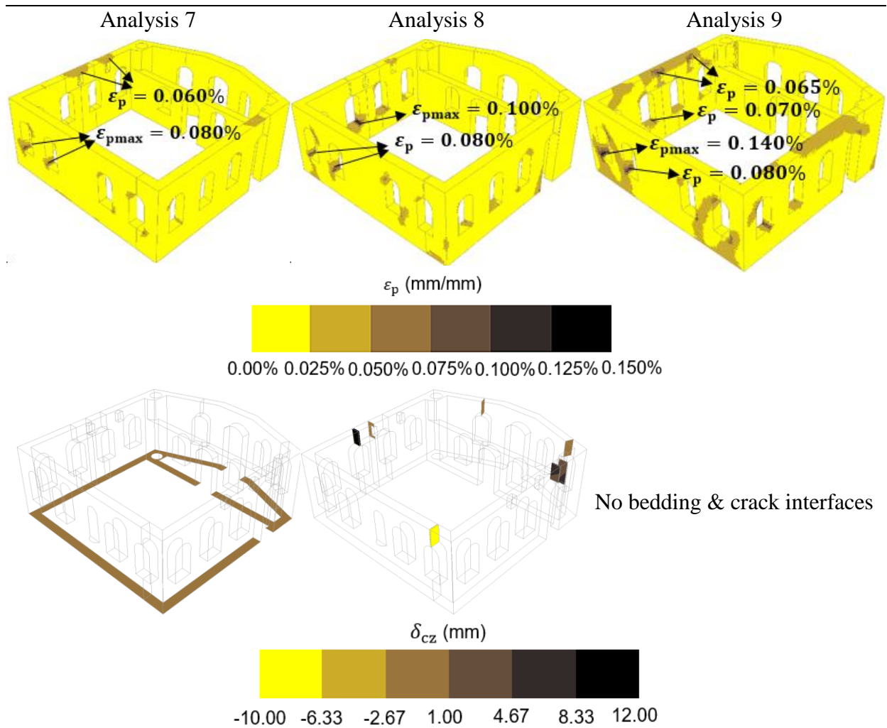
Fig. 17: The results of the Analyses 7, 8 and 9 (Variations of pre-existing cracks and bedding)
