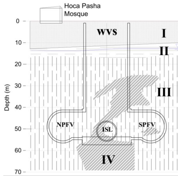
Fig. 3: Sectional view of the excavation site and geological sections (A-A section in Fig. 2a) (modified from Method Statements for Excavation and Support Works, 2008).
