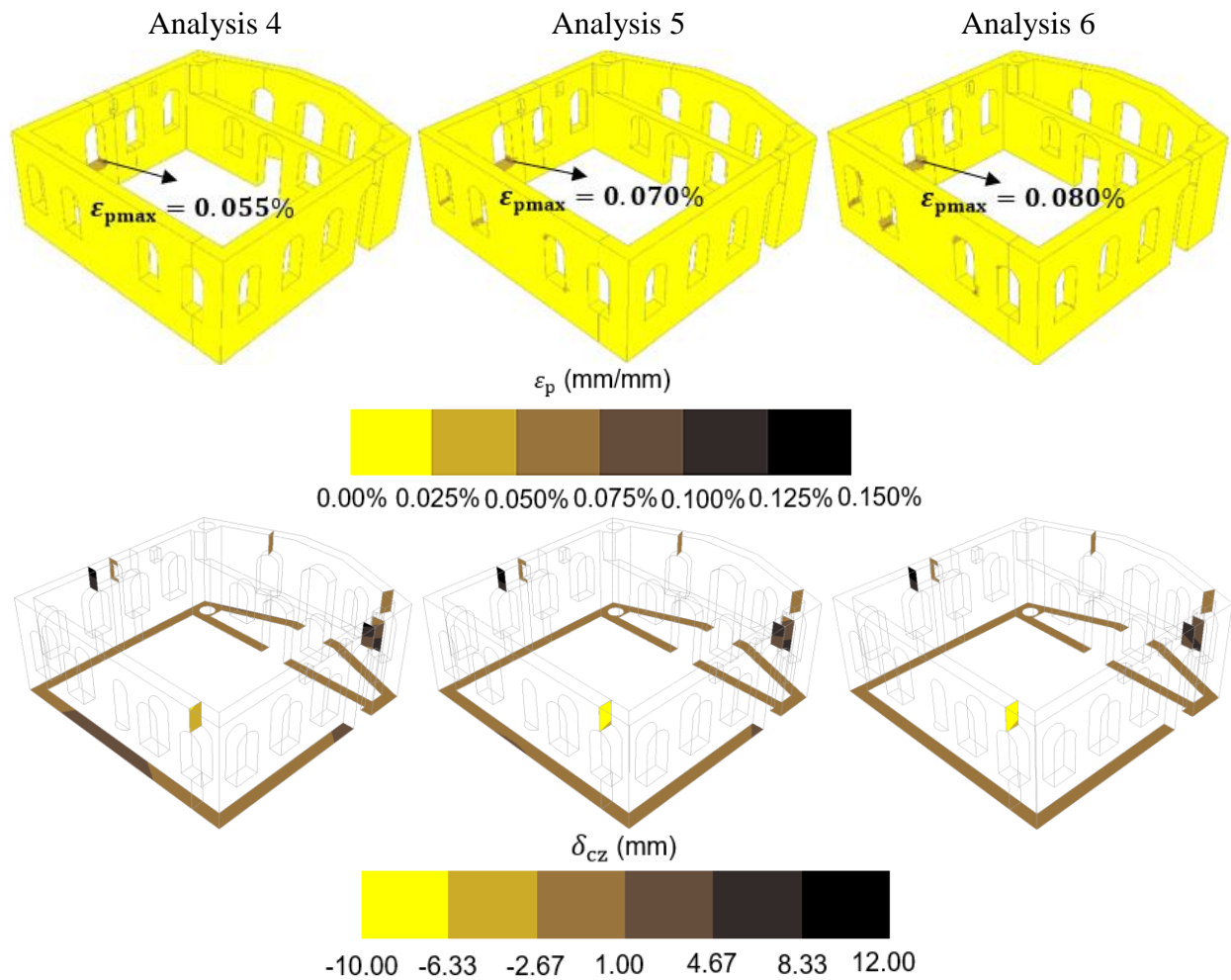
Fig. 16: The results of the Analyses 4, 5 and 6 (Variation of the bedding stiffness)
