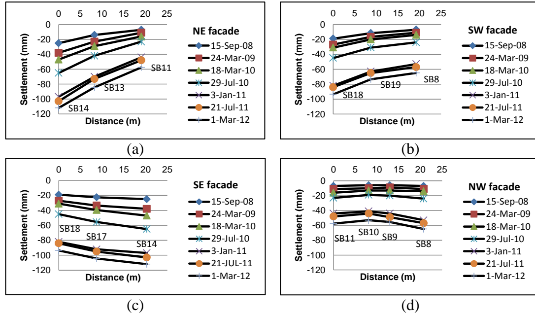
Fig. 7: Monitored settlements along the main masonry walls
