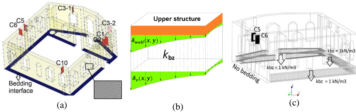
Fig. 9: (a) Mosque model geometry (b) Interface model and (c) interface configuration for the isolated SW wall
