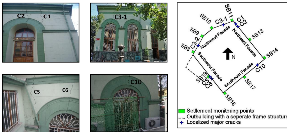
Fig. 5: The pre-existing localized cracks and their locations in the plan of the mosque
