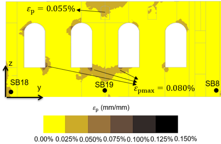
Fig. 10: \epsilon_p distribution in SW without C5 and C6 crack interfaces ( E_m = 350 MPa)
