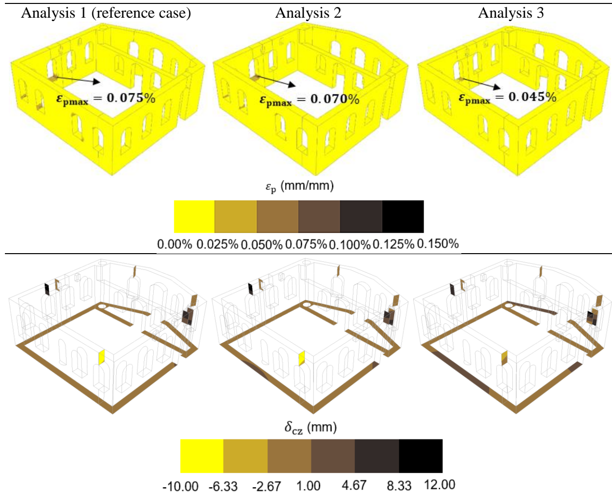
Fig. 15: The results of the Analyses 1, 2 and 3 (Variation of the masonry stiffness)
