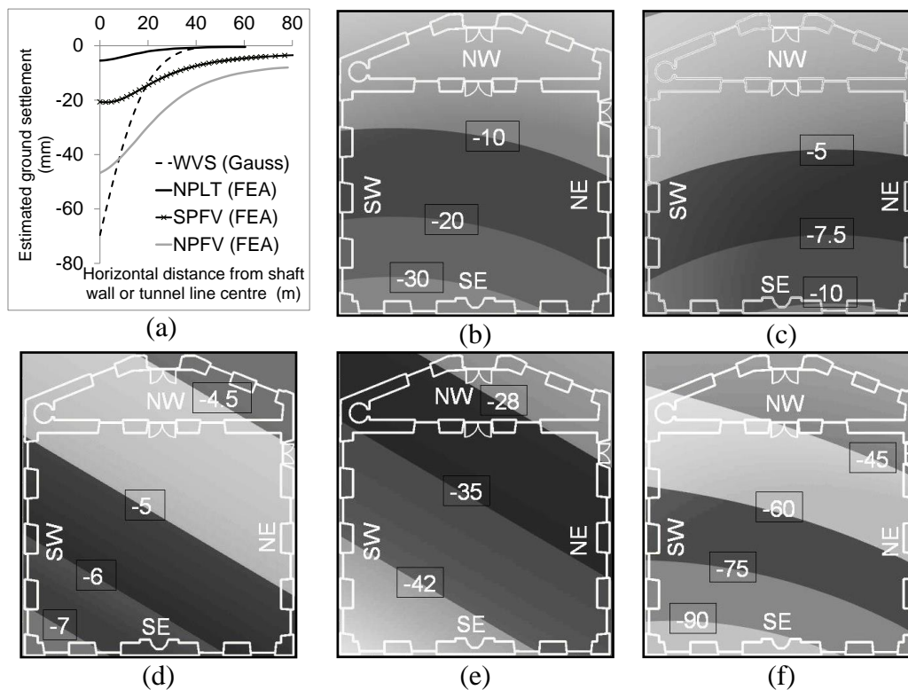
Fig. 13: (a) Reported or derived 2D free-field ground settlement estimations which are used to produce settlement fields and 3D settlement field contours generated for (b) WWS, (c) NPLT, (d) SPFV, (e) NPFV and (f) combination of WWS, NPLT, SPFV and NPFV excavations
