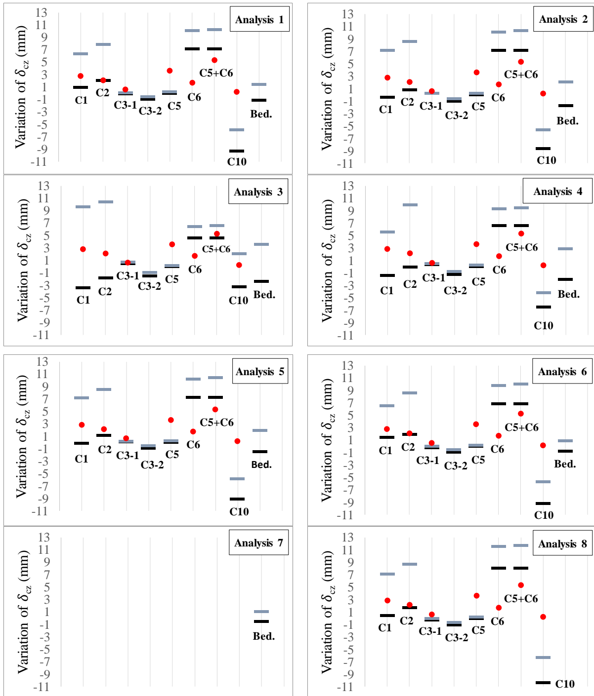
Fig. A.1: The ranges of variation of relative displacements of crack and bedding interfaces
