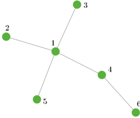
Figure 5.10: The resulting network after a simulation with the parameters \beta = 0.9, I_l = 0.5 .
