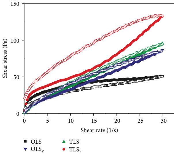
FIGURE 4: Rheogram of the systems studied, where OLS is opaque liquid system, OLS v is RP-loaded opaque liquid system, TLS is transparent liquid system, and TLS v is RP-loaded transparent liquid system. The solid symbols represent the upper curves and the hollow symbols represent the lower curves.
