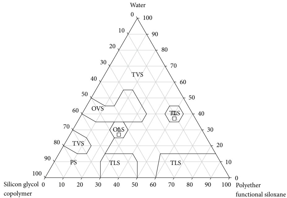
FIGURE 2: Ternary phase diagram, with O and the square (□) representing the selected regions, where TVS is transparent viscous system, OVS is opaque and viscous system, TLS is transparent liquid system, OLS is opaque liquid system, and PS is phase separation.
