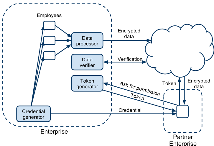
Figure 2.5: Cryptographic cloud storage, enterprise scenario.
