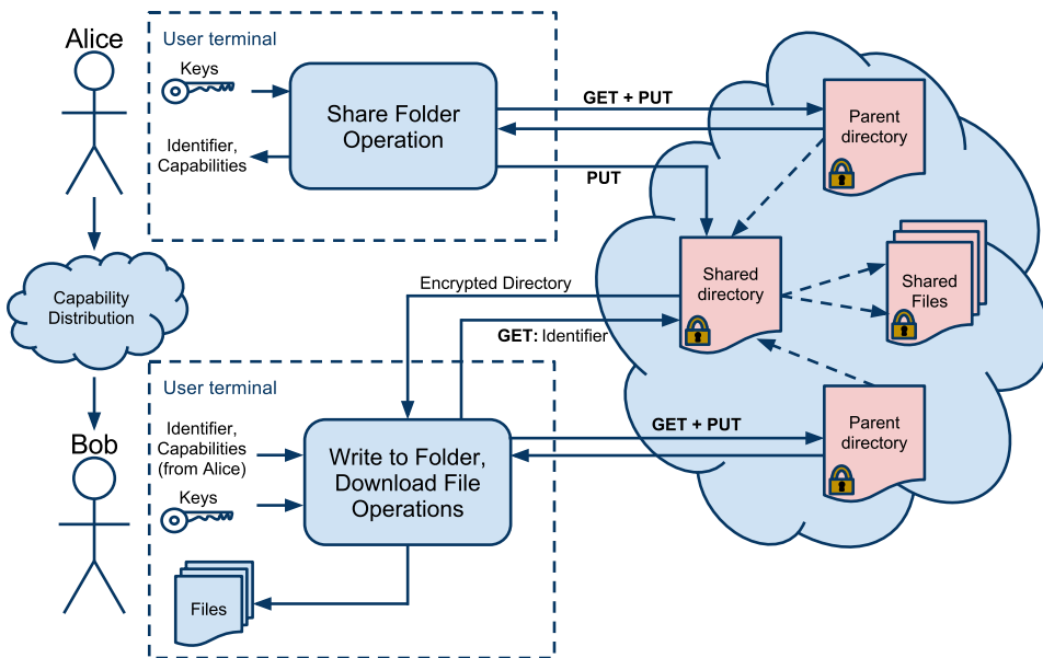
Figure 3.5: Scenario: Alice shares a file with Bob
