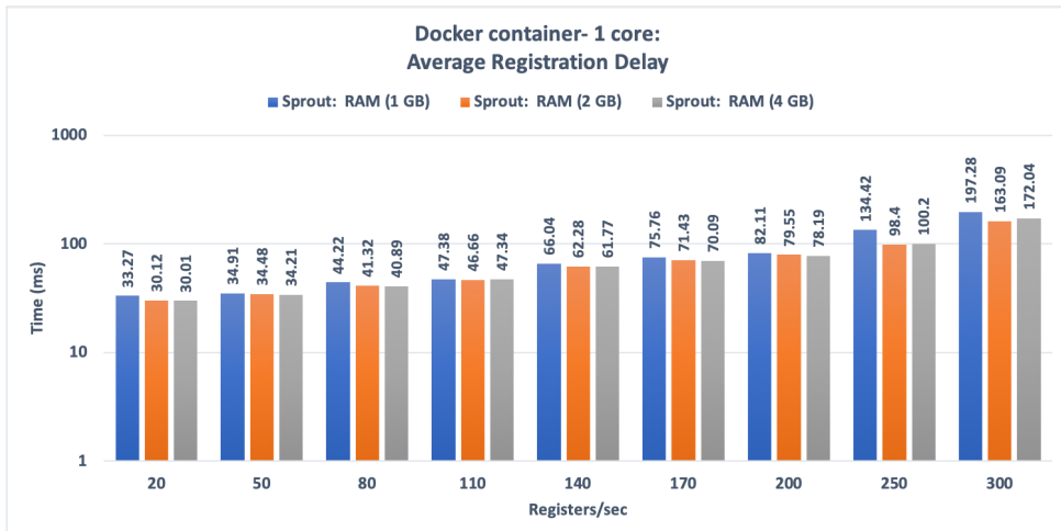
(b) Docker container: Average Registration Delay for Sprout with One Processing Core
