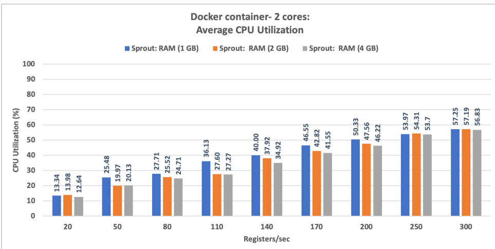
(b) Docker container: Average CPU Utilization for Sprout with Two Processing cores
