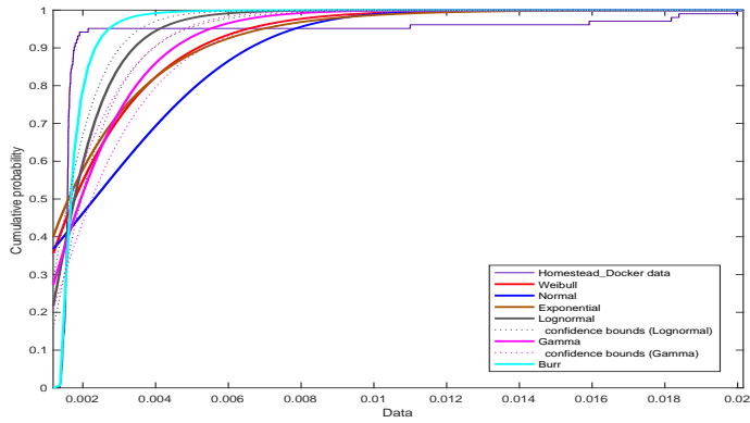
(c) Homestead: Service Time Distribution
