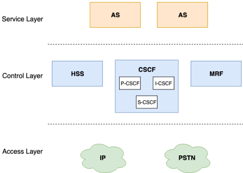
Figure 2.1: IMS High-level Architecture
