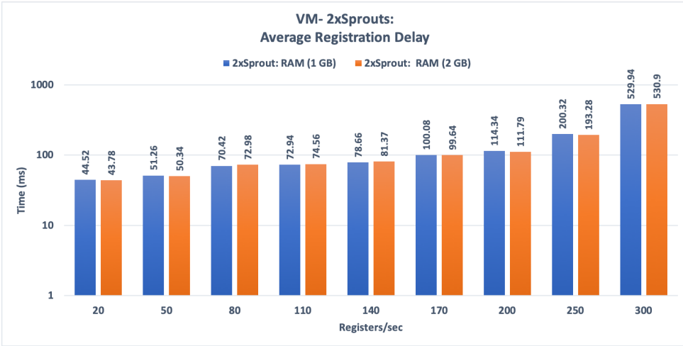
(a) VM: Average Registration Delay for 2xSprouts
