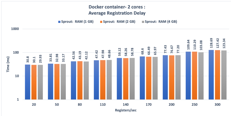
(b) Docker container: Average Registration Delay for Sprout with Two Processing Cores
