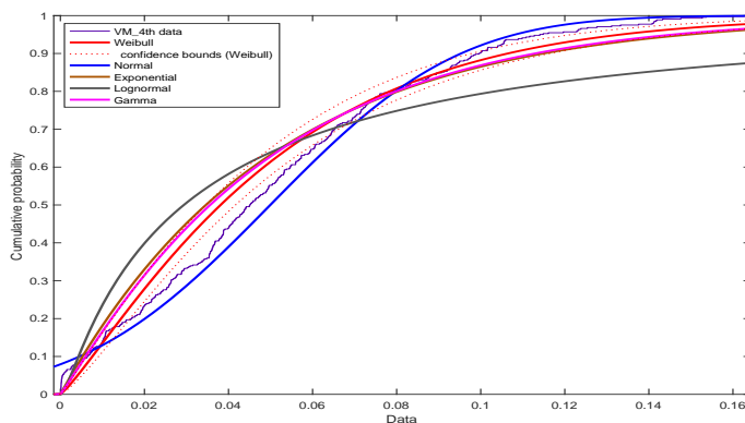
(c) VM: Bono Inter-Arrival Time Distribution
