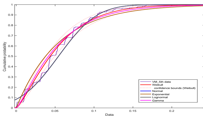
(a) Docker: Sprout Inter-Arrival Time Distribution
