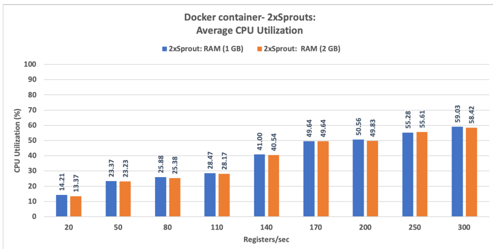
(b) Docker container: Average CPU Utilization for 2xSprouts
