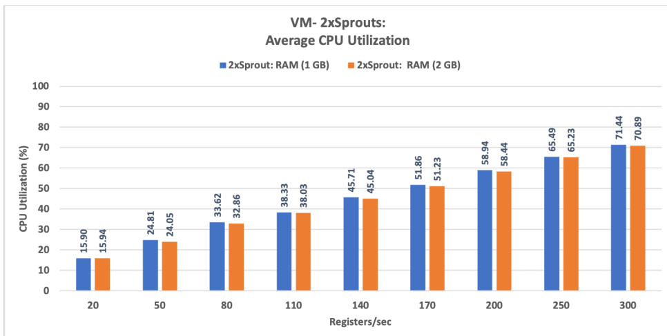
(a) VM: Average CPU Utilization for 2xSprouts
