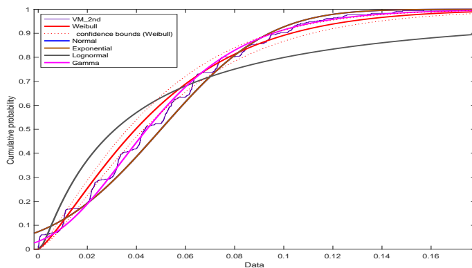
(a) VM: Homestead Inter-Arrival Time Distribution
