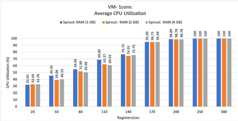
(a) VM: Average CPU Utilization for Sprout with One Processing Core
