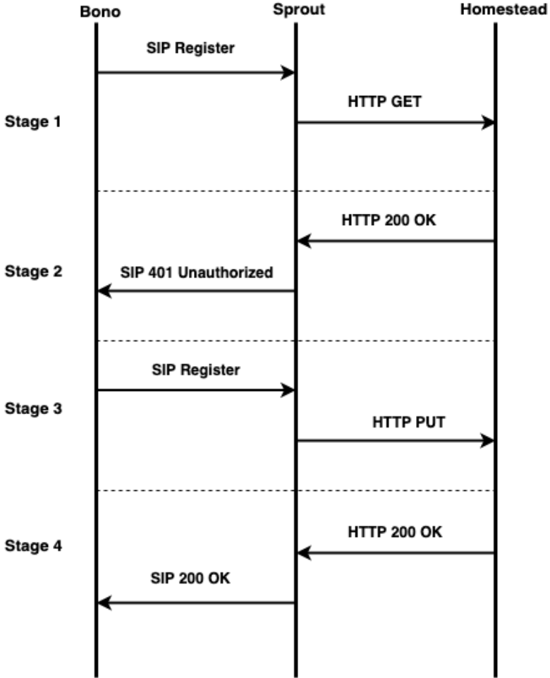
Figure 3.3: SIP: User Registration Dialogue, adapted from [Neta]
