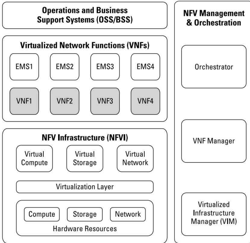
Figure 1.1: NFV high-level Architectural Framework, adapted from [ETS13a]
