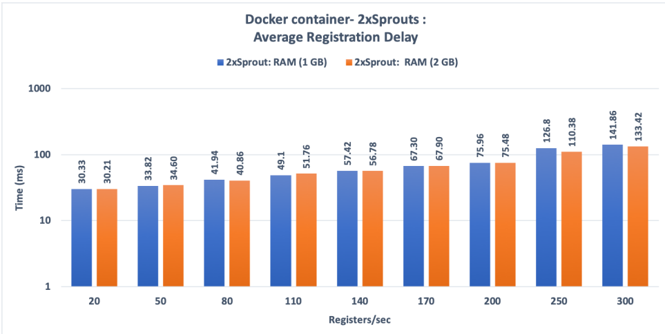
(b) Docker container: Average Registration Delay for 2xSprouts
