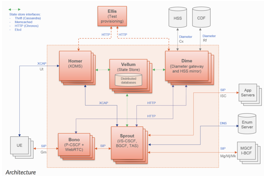
Figure 3.1: ClearWater Architecture, adapted from [Neta]
