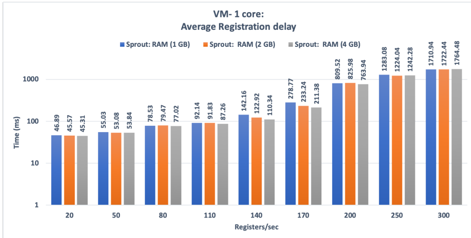
(a) VM: Average Registration Delay for Sprout with One Processing Core
