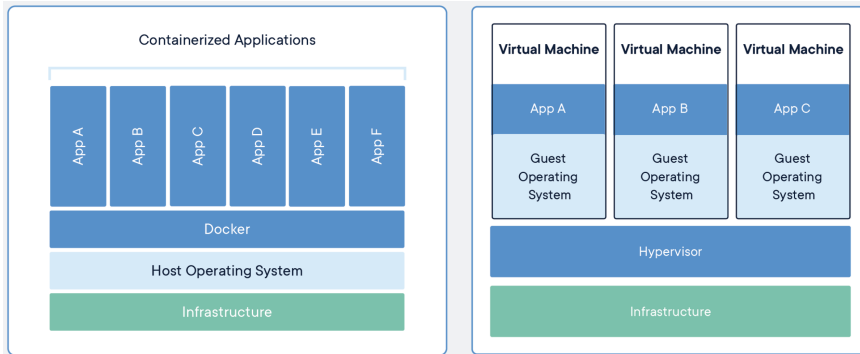
Figure 3.2: Container vs VM, adapted from [Doc18]
