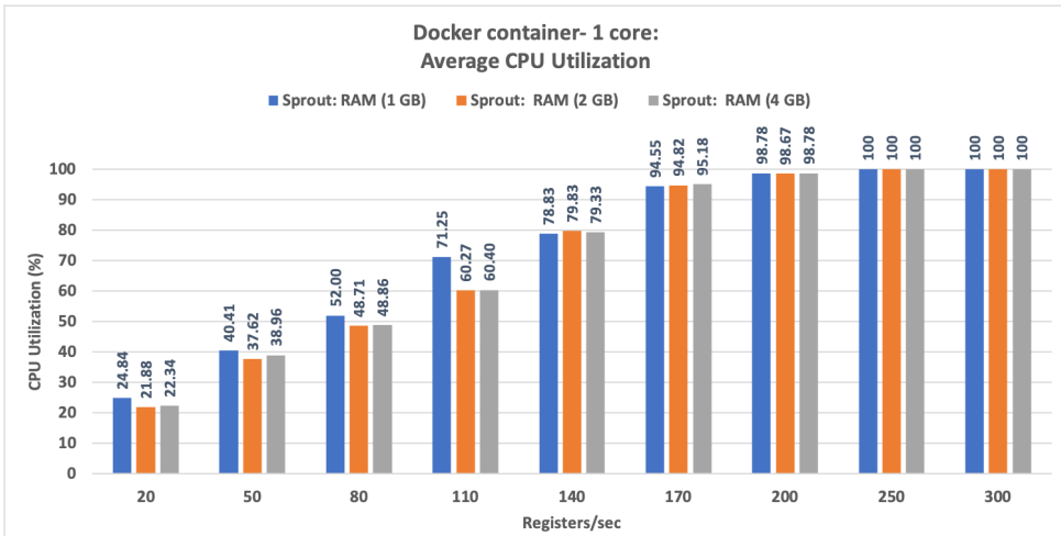
(b) Docker container: Average CPU Utilization for Sprout with One Processing Core
