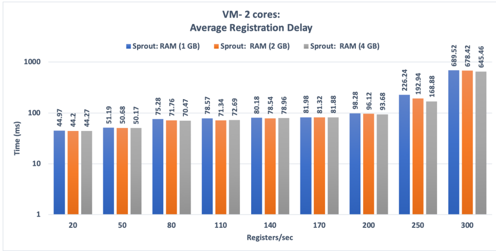
(a) VM: Average Registration Delay for Sprout with Two Processing Cores
